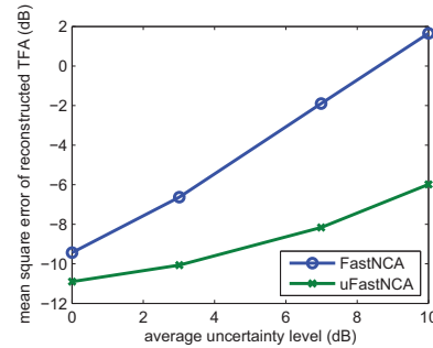
Figure 1 Simulation results on synthetic data
