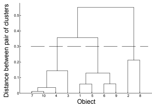
Fig. 12. A dendrogram for clustering ten objects.
