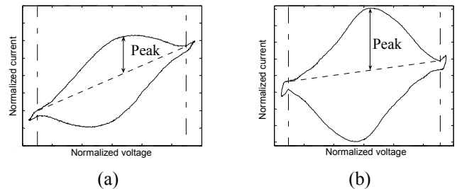
Fig. 11. The trajectories of (a) a radio, and (b) a CD player operating in stand by mode.
