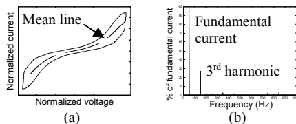
Fig. 5. (a) The trajectory of a vacuum cleaner and its mean line (dotted line); (b) the current spectrum of the vacuum cleaner.
