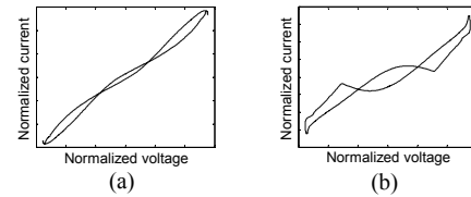
Fig. 6. (a) The trajectories of a window-type air conditioner, and (b) a microwave oven.
