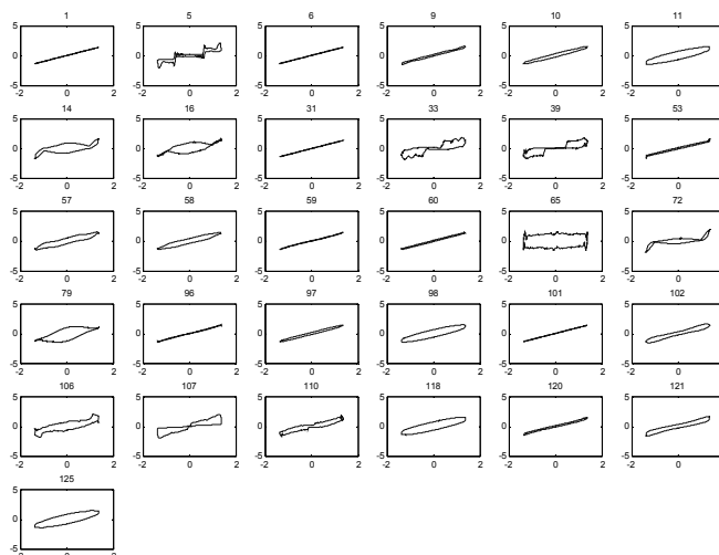
Fig. 15. The V-I trajectories of the Group 3 appliances in the taxonomy based on traditional power metrics.
