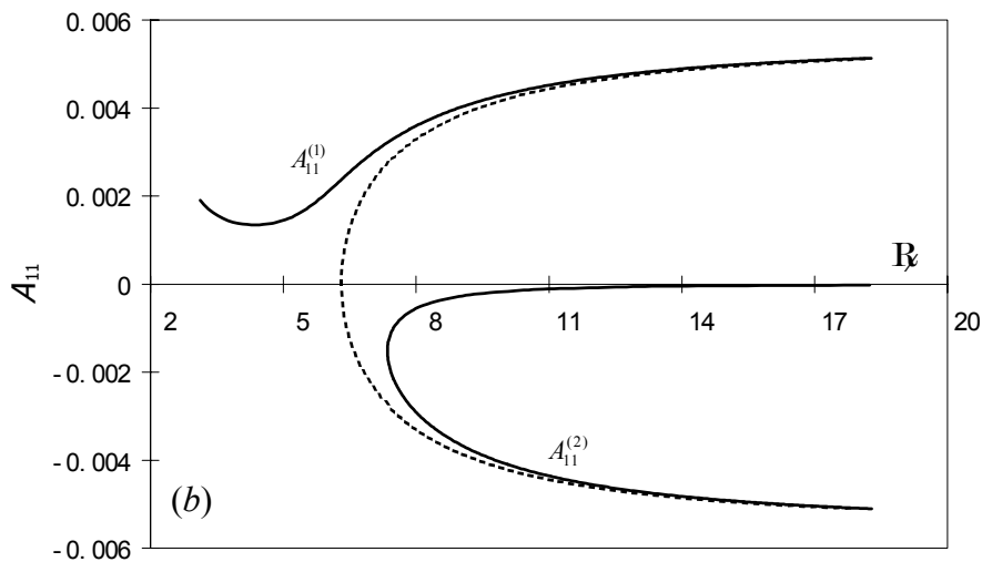
Figure 6b. Fundamental resonance as \mathbb{W} \approx \omega_{20} , — denotes forced response curve and - - denotes backbone curve.
