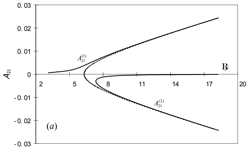
Figure 6a. Fundamental resonance as \mathbb{W} \approx \omega_{20} , — denotes forced response curve and - - denotes backbone curve.
