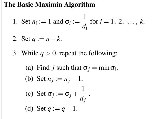
Figure 1: The Basic Maximin Algorithm
