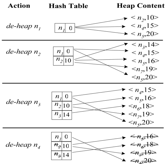
Fig. 6. Hash table and heap contents.
