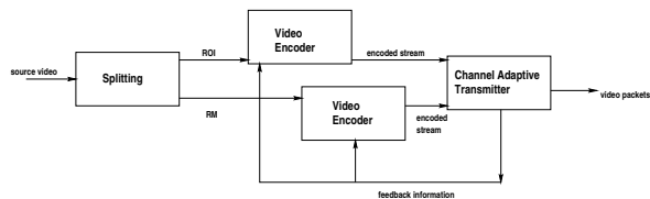
Fig. 1. The proposed channel adaptive video transmission scheme.
