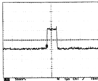
Fig. 4 Rectangular pulse response of the LED. The LED is intensity-modulated by a 1 μs rectangular pulse. The turn-on and turn-off time are both found to be 50 ns.
