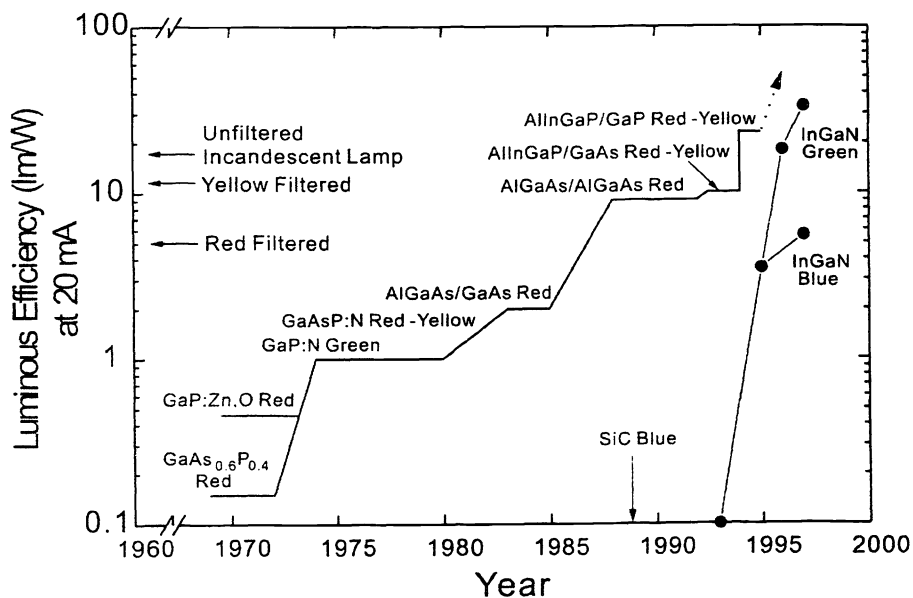
Fig. 1 Evolution of visible LED technology and performance. Luminous efficiencies of unfiltered and filtered incandescent lamps are included for comparison.
