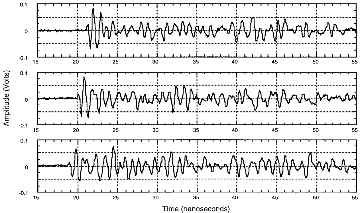
Fig. 10. Averaged multipath profiles in a 40 ns window, measured in an office along the horizontal cross section of the grid at three different aligned positions of 18 in. apart. The transmitter is approximately 6 m from the receiver, representing typical UWB-signal transmissions for the "high signal-to-noise ratio" environment.
