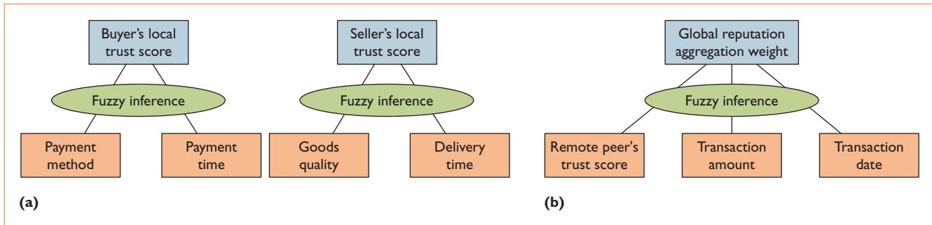
Figure 3. Local trust inference versus global reputation aggregation. The FuzzyTrust system (a) performs fuzzy logic inferences to determine the local trust scores and (b) uses accumulated local scores for weight inference in global reputation aggregation.
