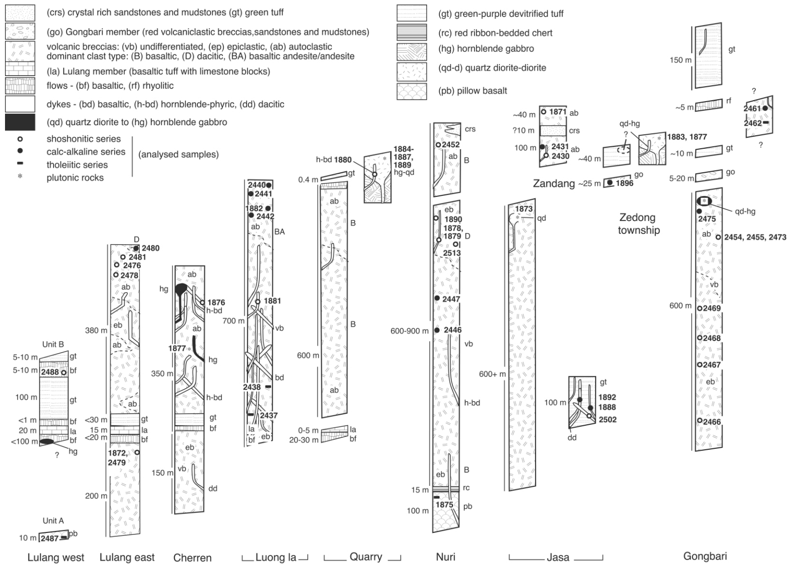
Figure 2. Reconstructed stratigraphic sections compiled from mapping traverses across the Zedong terrane (McDermid 2002), showing the stratigraphic levels from which samples were collected.
