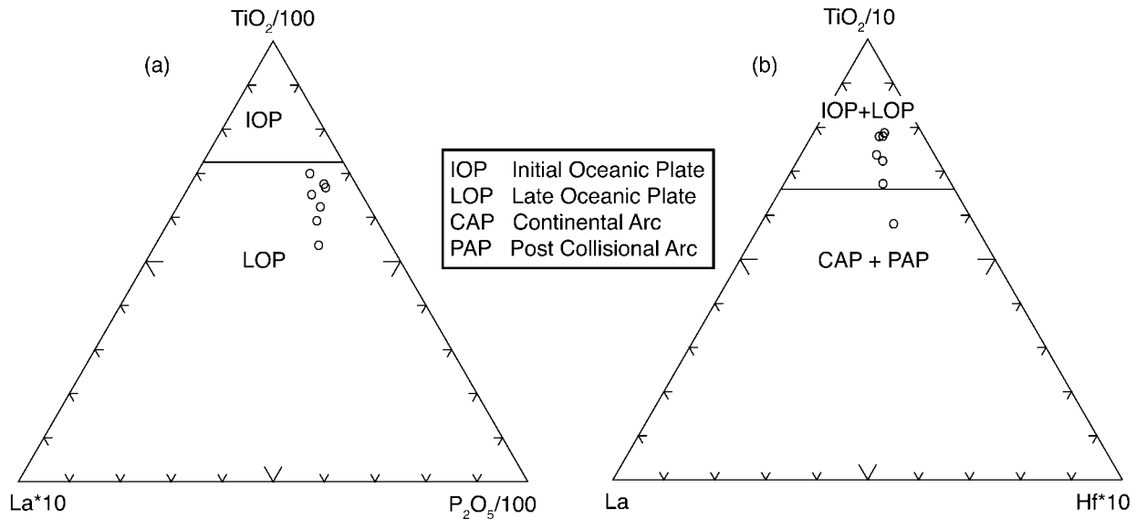
Figure 8. Zedong terrane sample data plotted on ternary trace element discrimination diagrams for potassic igneous rocks. Fields and sample screening criteria after Müller et al. (1992).
