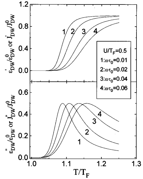
FIG. 9. Complex dielectric constant \epsilon_{DW} = \epsilon'_{DW} - i\epsilon''_{DW} and complex compliance J_{DW} = J'_{DW} - iJ''_{DW} ( Q^{-1} = J''_{DW}/J'_{DW} ) related to domain freezing versus temperature T calculated from Eqs. (7) and (9) with one set of U and \tau_0 at different frequency \omega (= 2\pi f) .
