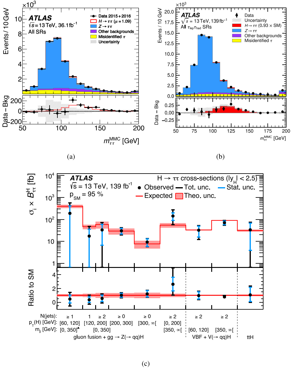
Fig. 12. (a) The invariant mass of the \tau\tau system for all combinations of \tau -lepton decays using 36.1 fb ^{-1} of data [123]. (b) The same observable considering only signal regions with one \tau -lepton decaying leptonically and one decaying hadronically for 139 fb ^{-1} of data [125]. (c) The measured cross-sections times branching ratio in nine different kinematic regions compared with the SM expectations [125].
