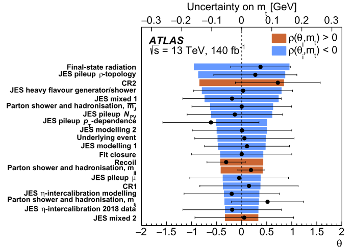
Fig. 3. The contribution of individual NPs, \theta , to the total uncertainty in m_t is shown by the coloured bars and can be read off using the upper x -axis. The red (blue) coloured bars represent NPs that have a positive (negative) correlation with m_t and only NPs that have a contribution to the uncertainty in m_t of more than 0.05 GeV are shown. The fitted values and post-fit uncertainties for these NPs are shown by the points, which refer to the lower x -axis. All modelling uncertainties displayed in the figure correspond to uncertainties in the t\bar{t} process.
