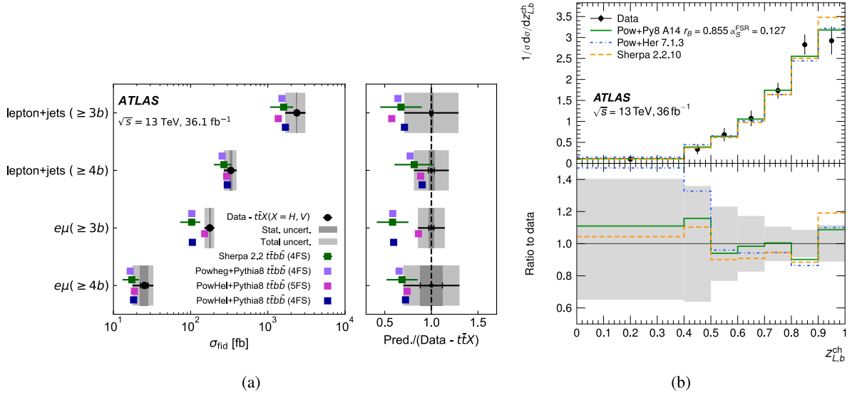
Fig. 6. (a) Measured fiducial \bar{t}\bar{t} + b -jet cross-sections [103], with \bar{t}\bar{t}H and \bar{t}\bar{t} -plus-vector-boson contributions subtracted from the data, compared with predictions from different generator set-ups. (b) Particle-level differential cross-section as a function of z_{L,b}^{\text{ch}} [104], compared with predictions from different generator set-ups. The quantity z_{L,b}^{\text{ch}} is defined as the fraction of the total charged-particle momentum in a jet carried by the b -hadron decay products along the direction of the jet.
