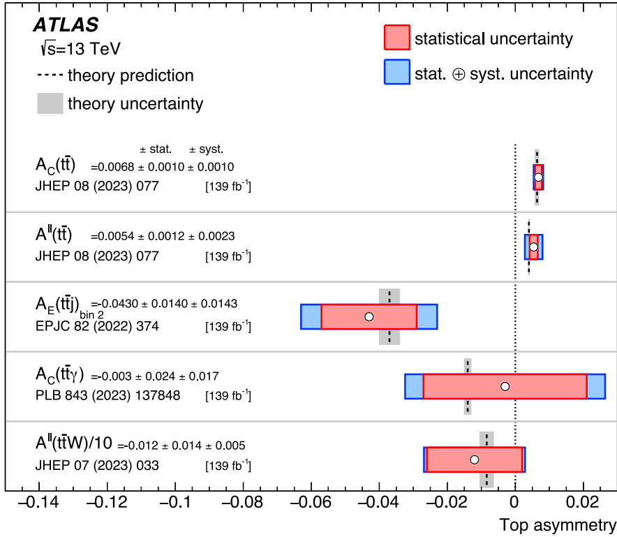
Fig. 13. Summary of the \sqrt{s} = 13 TeV top asymmetry measurements using the full Run 2 dataset: t\bar{t} asymmetry, lepton-based asymmetry, energy asymmetry in the bin with the largest expected asymmetry, and asymmetry in t\bar{t}\gamma and t\bar{t}W events. Each of the results is compared with their corresponding theoretical expectation. The value of the t\bar{t} asymmetry in t\bar{t}W events is shown divided by 10 for display purposes.
