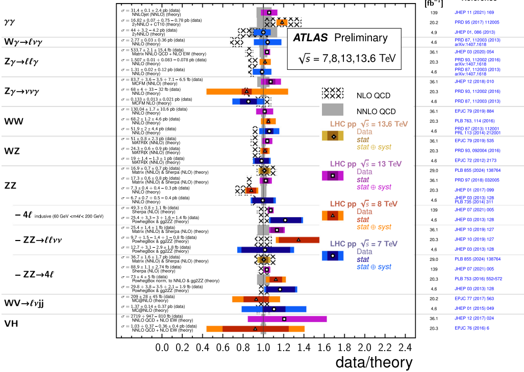
Fig. 24. Overview of ATLAS diboson cross-section measurements. The results discussed in this review are shown with a square marker [134].
