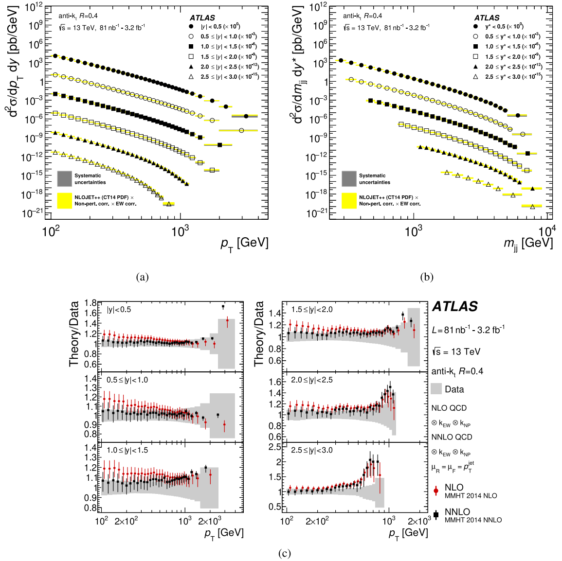
Fig. 8. The measured (a) inclusive jet and (b) inclusive dijet cross-sections at \sqrt{s} = 13 \text{ TeV} , shown as a function of the jet transverse momentum or dijet invariant mass in several jet rapidity bins [64]. (c) The ratios of NLO and NNLO pQCD predictions [66–68] to the measured inclusive jet cross-sections. The theory uncertainties are shown by the lines and the shaded bands show the total data uncertainty including both the systematic and statistical uncertainties.
