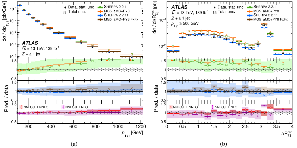
Fig. 19. Z +jets cross-section as a function of (a) the p_T of the leading jet and (b) the angle between the Z and the closest jet for events with p_{T,j1} > 500 GeV [154]. The lower panels show the ratios of the predictions [4,6,7,9,155,156] to the data.
