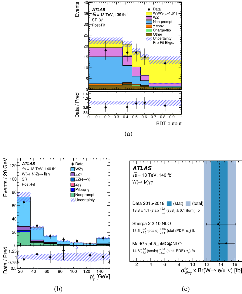
Fig. 36. (a) Post-fit WWW BDT score in the 3-lepton channel [248], (b) distribution of photon E_T in the WZ\gamma SR [249] and (c) the measured fiducial W(\rightarrow e\nu/\mu\nu)\gamma\gamma integrated cross-section compared with theory predictions [247]. The lower panels show the ratios of the data to the predictions [6,7].
