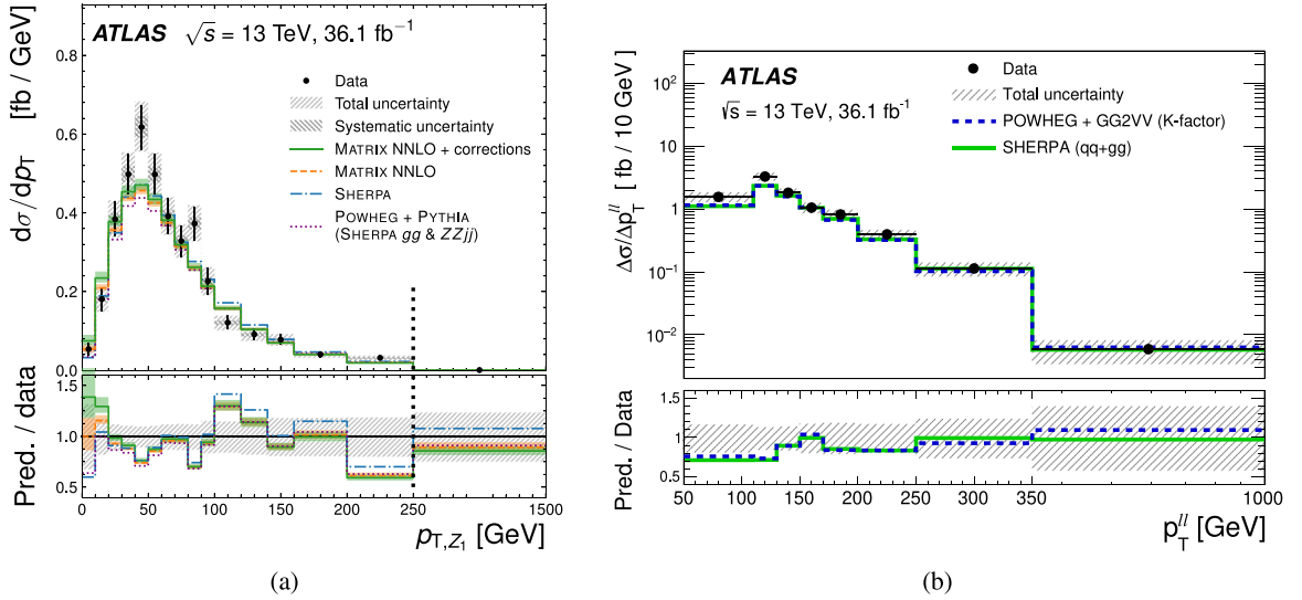
Fig. 27. Differential cross-sections as a function of (a) p_{T,Z1} in llll final states [209] and (b) p_T^{ll} in ll\nu\nu final states [210]. The lower panels show the ratios of the predictions [6,58,193,195,212] to the data.
