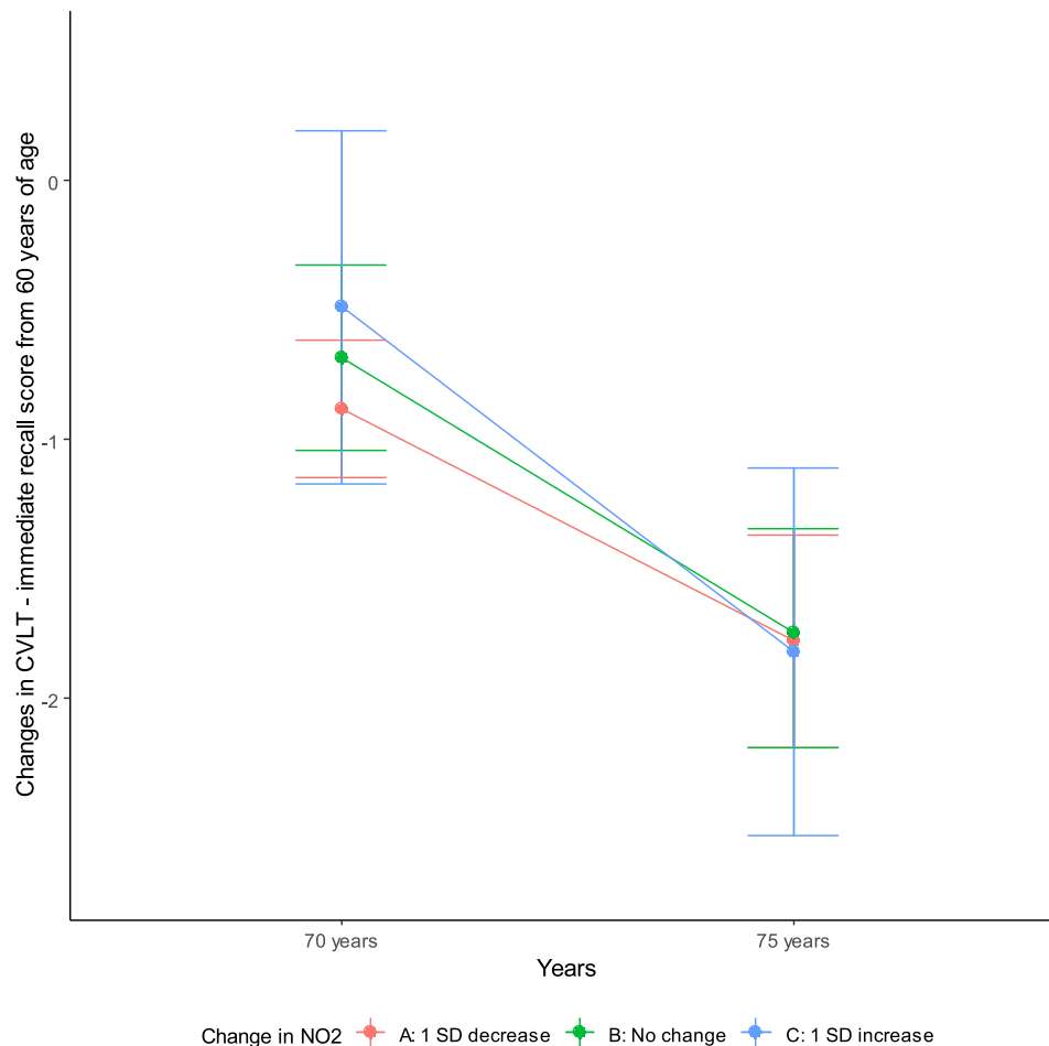
Fig. 3. Moderating effects of changes in annual average concentrations of NO 2 on changes in CVLT – immediate recall score from 60 years of age (direct effect model estimates).
