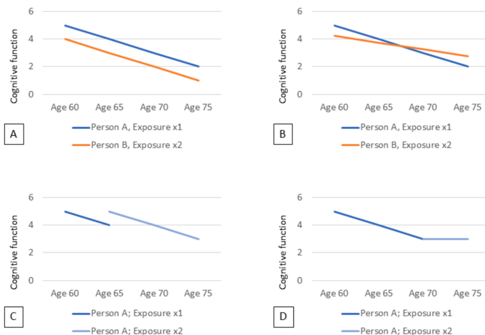
Fig. 2. Interpretation of effects of neighbourhood environmental attributes on cognitive function examined in this study. Panel A: person-level average exposure as a correlate of person-level cognitive function; panel B: person-level average exposure as a correlate of person-level trajectories of cognitive function (i.e., exposure as a moderator of trajectories); panel C: within-person change in exposure as a correlate of within-person change in cognitive function level; panel D: within-person change in exposure as a correlate of within-person changes in trajectory of cognitive function (i.e., change in exposure as a moderator of trajectories). Exposure level x_2 is presented as being more beneficial than x_1 in all graphs except for panel A.
