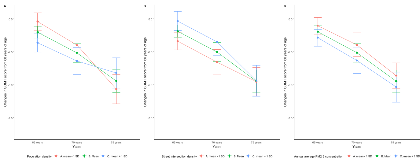
Fig. 4. Moderating effects of environmental attributes on changes in Symbol Digit Modalities Test (SDMT) scores from 60 years of age. Direct effect estimates for person-level average population density (panel A), street intersection density (panel B) and average annual concentrations of PM 2.5 (panel C).
