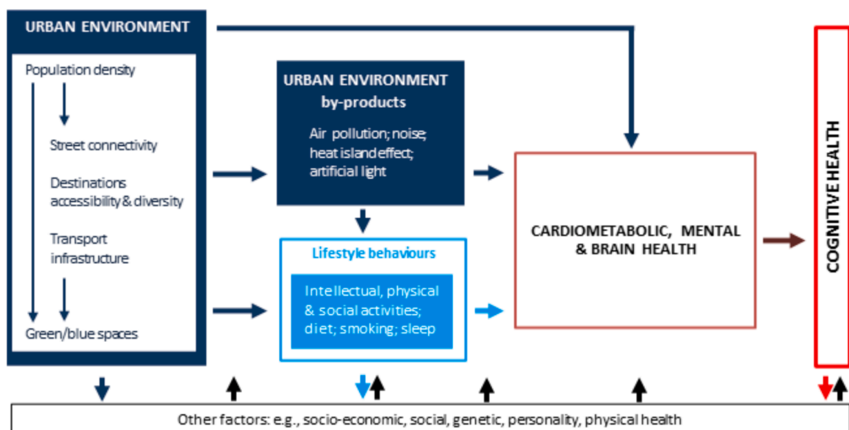
Fig. 1. A simplified ecological model of urban neighbourhood environmental influences on cognitive health.
