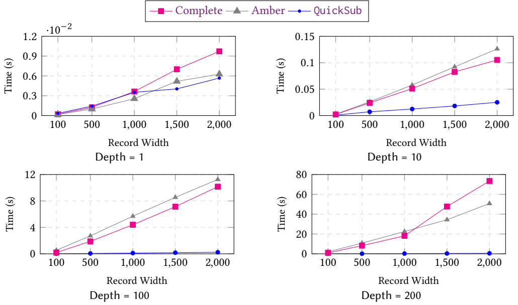
Fig. 12. Runtime results (seconds) for different algorithms with varying benchmark sizes in depth and width.
