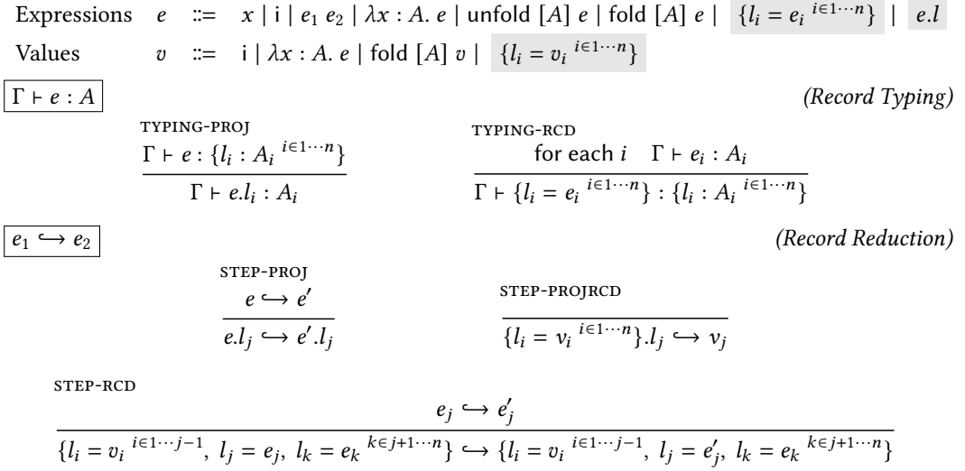
Fig. 7. Extension to record expressions.
