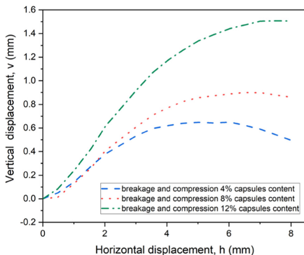
Fig. 9 Volumetric response from particle movement and capsules breakage and compression. (vertical stress of 30 kPa, capsules content of 4%, 8%, and 12%)
