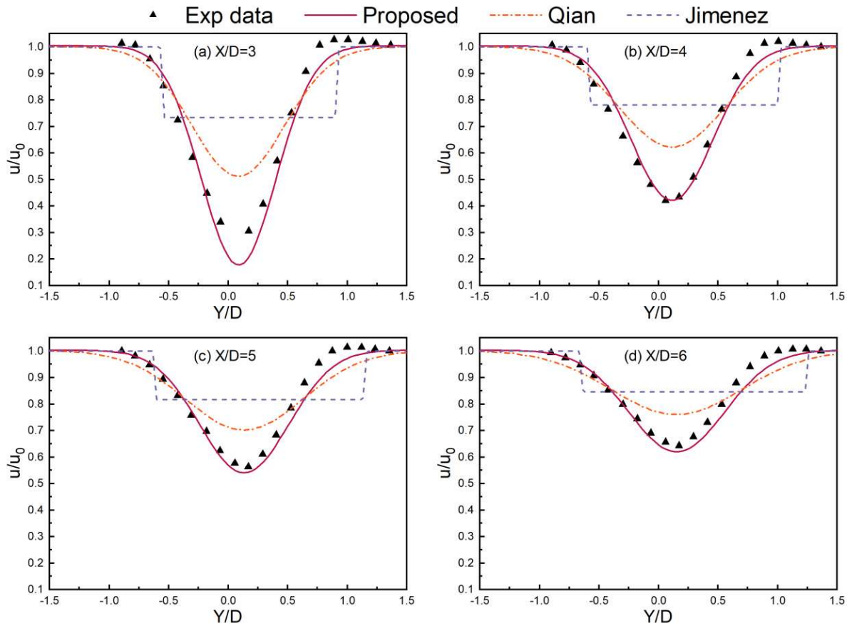
Fig. 3 Deflected wake distribution with a yaw angle of 10°.
