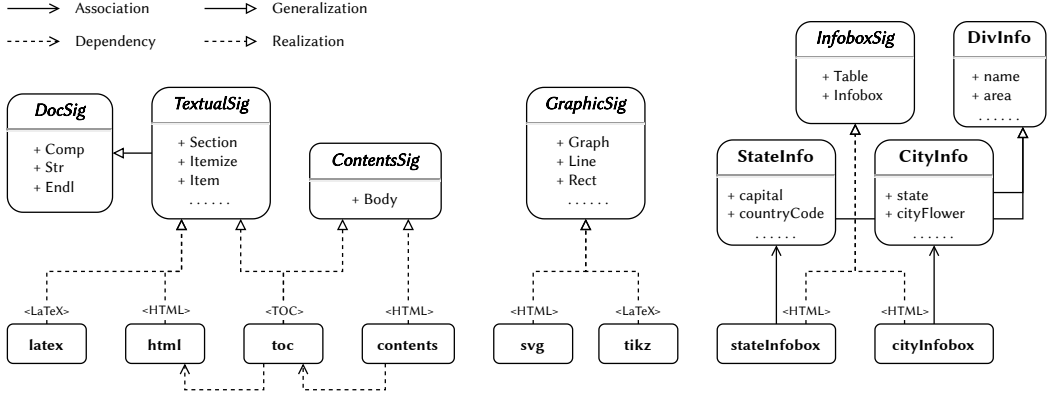
Fig. 4. A simplified diagram of ExT components.
