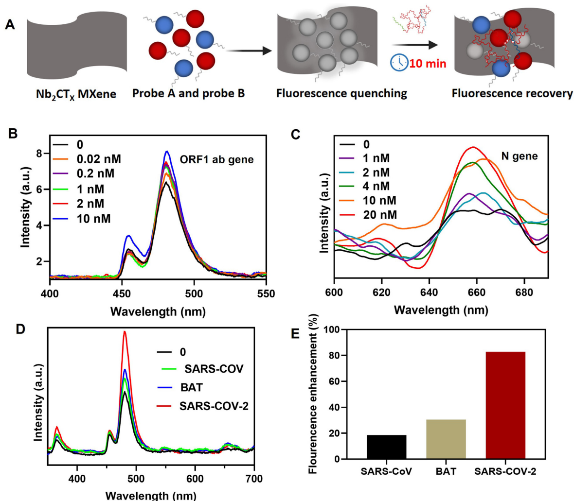
Fig. 4. (A) The scheme of detection of long simulated target using dual emission UCNPs/MXene integrated biosensor. Photoluminescence spectra at different emission bands of the proposed biosensor for simultaneous multiplexed detection of (B) ORF-1ab and (C) N -target. (D) PL intensity recovery comparison for RNA-targeted regions among three highly homologous coronavirus. (E) The specificity analysis of the using dual emission UCNPs /MXene integrated biosensor.
