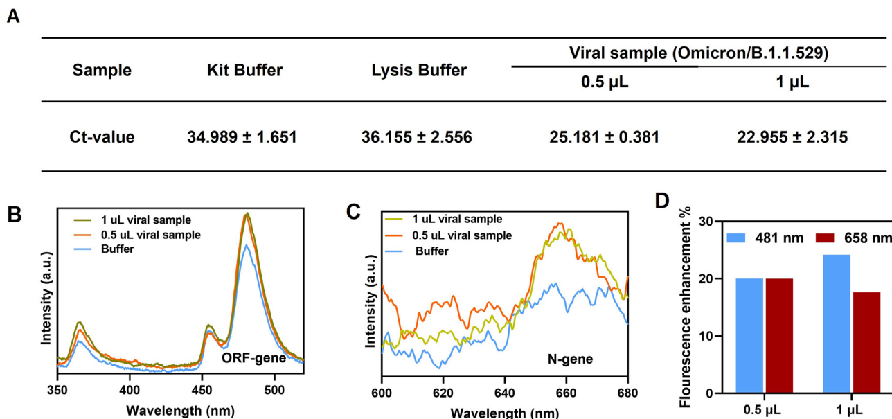
Fig. 5. (A) RT-qPCR results of ORF-gene in different volume viral samples (different amount viral samples serve as positive control groups, while the kit buffer and lysis buffer without virus and serves as negative control groups). (B) Blue emission and (C) red emission of UCNPs/MXene integrated biosensor when adding viral sample (0.5 \mu L and 1 \mu L of SARS-CoV-2 Omicron/B.1.1529 stock solution extracted from cells, sample to answer time: 5 min). (D) Peak intensities enhancement of the Nb 2 CT x /UCNP integrated biosensor after probing different quantities of viral samples, corresponding to (B) and (C). (For interpretation of the references to color in this figure legend, the reader is referred to the web version of this article.)
