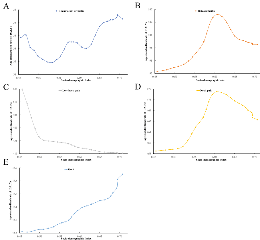
Fig. 2 Correlation of age-standardized rate of DALYs with SDI for five major musculoskeletal disorders between 1990 and 2017. Correlation of age-standardized rate of DALYs with SDI for rheumatoid arthritis (a), osteoarthritis(b), low back pain(c), neck pain (d), and gout (e). SDI sociodemographic index
