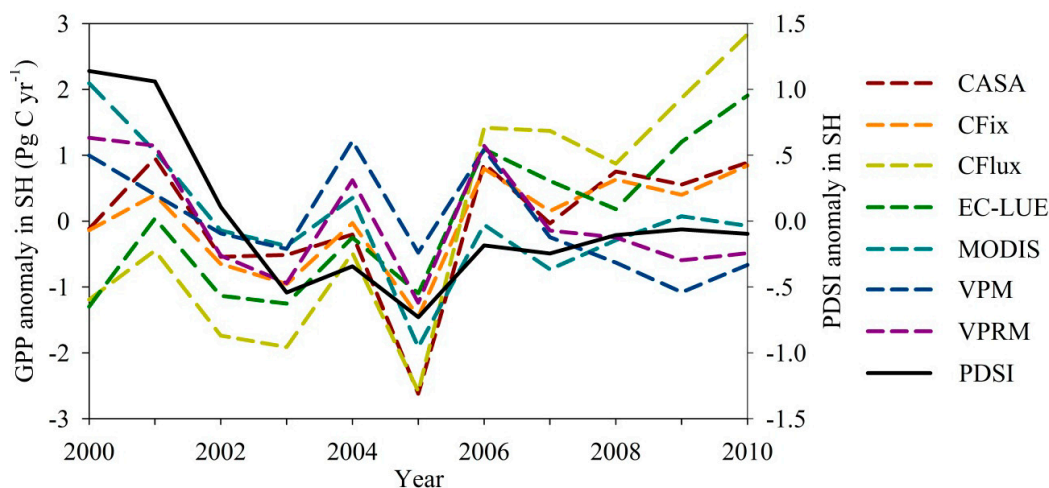
Figure 4. Interannual variations of annual GPP estimates and PDSI over the Southern Hemisphere (SH).
