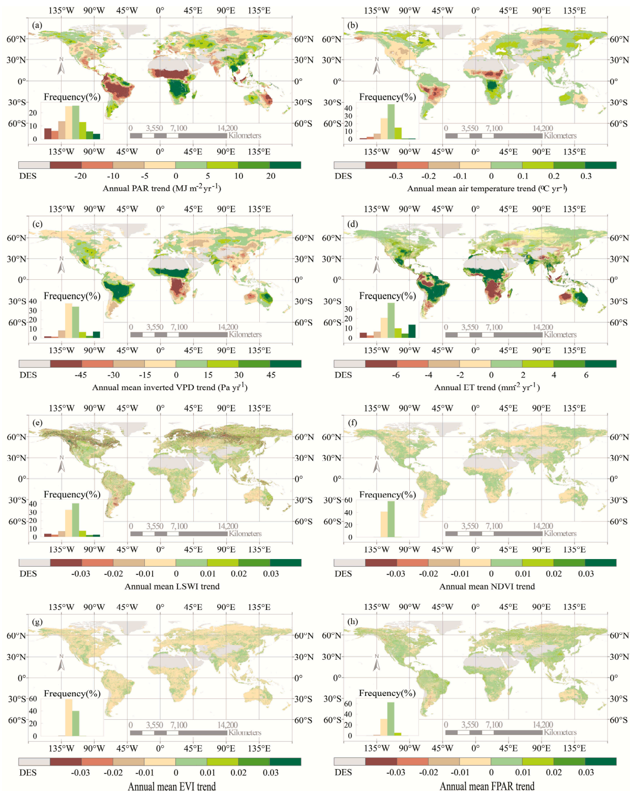
Figure 6. Spatial patterns on the change trends of environmental variables and vegetation indices: (a) Photosynthetically Active Radiation (PAR); (b) air temperature ( T_a ); (c) inverted Vapor Pressure Deficit (VPD); (d) evapotranspiration (ET); (e) Land Surface Water Index (LSWI); (f) Normalized Difference Vegetation Index (NDVI); (g) Enhance Vegetation Index (EVI); and (h) the Fraction of PAR absorbed by the vegetation canopy (FPAR). DES is no vegetation area.
