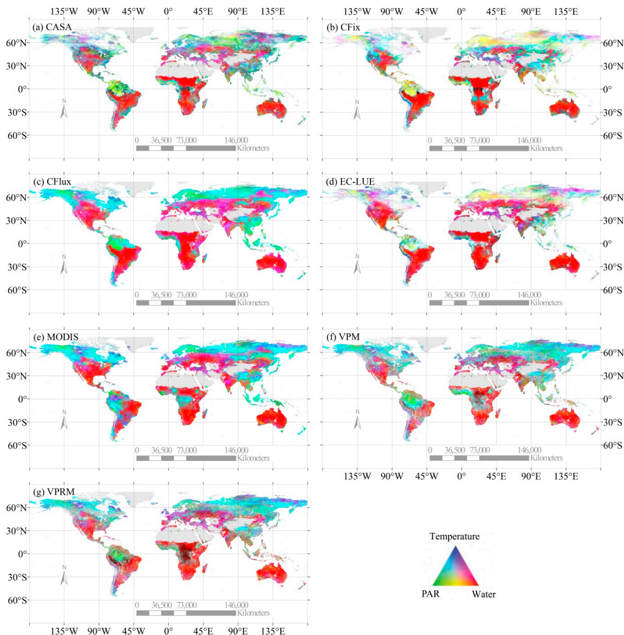
Figure 5. Spatial distribution of the environmental constraints to the annual GPP estimates over the period 2000–2010 of seven LUE models: (a) CASA; (b) CFix; (c) CFlux; (d) EC-LUE; (e) MODIS; (f) VPM; and (g) VPRM. Three environmental variables were considered: solar radiation (PAR, Green), air temperature (Blue), and water availability (Red).
