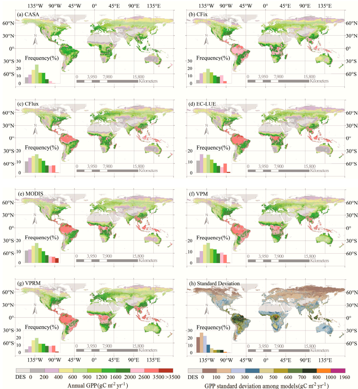
Figure 1. Spatial patterns of the global annual GPP estimates over the period 2000–2010 by (a) CASA; (b) CFix; (c) CFlux; (d) EC-LUE; (e) MODIS; (f) VPM; and (g) VPRM models; (h) the standard deviation of the GPP estimates among models. DES is no vegetation area.
