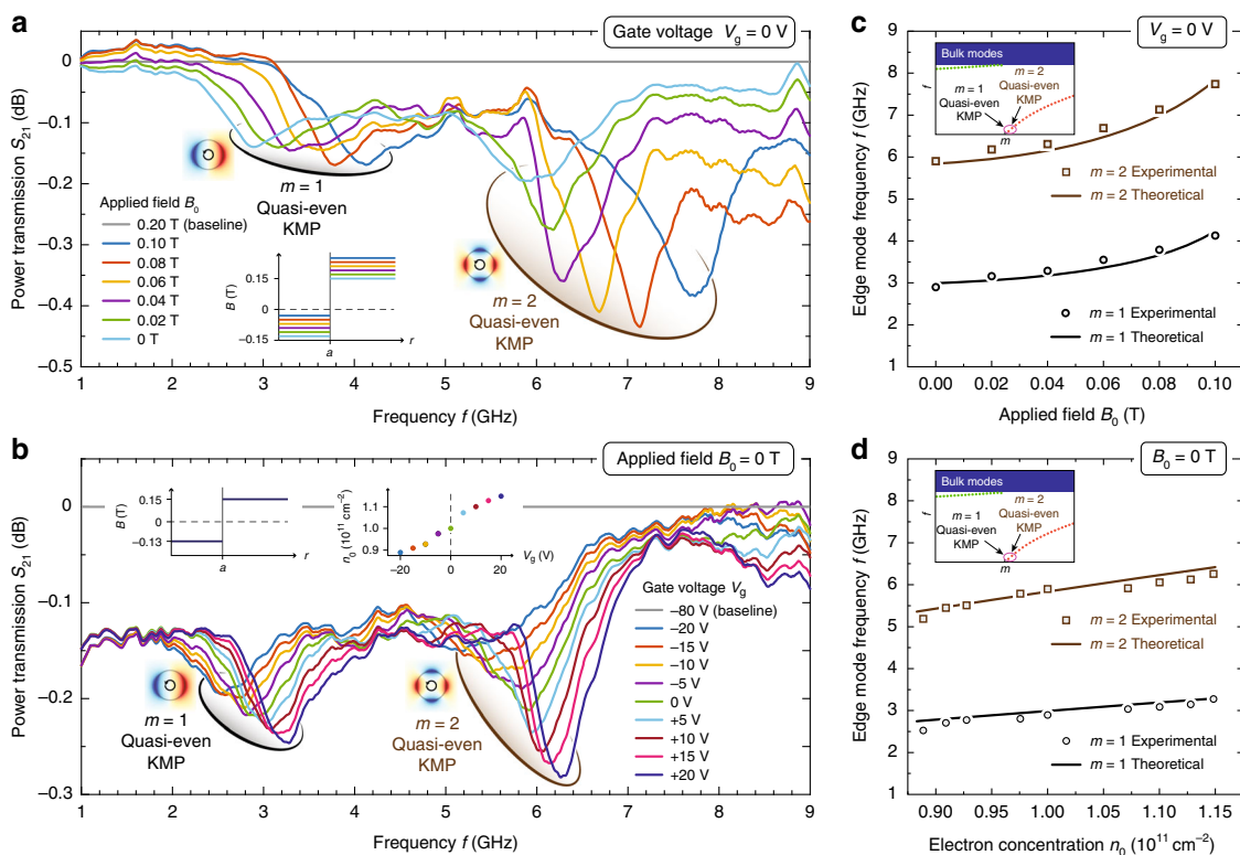
Fig. 3 Experimental observation of topological kink magnetoplasmons (KMPs). a and b Measured power transmission S_{21} (normalized to indicated baselines) as a function of frequency for a , varying applied uniform fields B_0 ( V_g = 0 V) and b , varying gate voltages V_g ( B_0 = 0 T). The characteristic absorption dips correspond to quasi-even KMPs with angular wavenumber m = 1 and 2, as indicated. Insets depict the (idealized) total magnetic field profile B(r) across the domains, as well as the measured dependence of the electron concentration n_0 with V_g (from independent Hall transport measurements). c and d Comparison between experimental observations and theoretical calculations. Dependence of KMP frequencies with c , applied field B_0 ( V_g = 0 V, n_0 = 1 \times 10^{11} \text{ cm}^{-2} ) and d electron concentration n_0 ( B_0 = 0 T)
