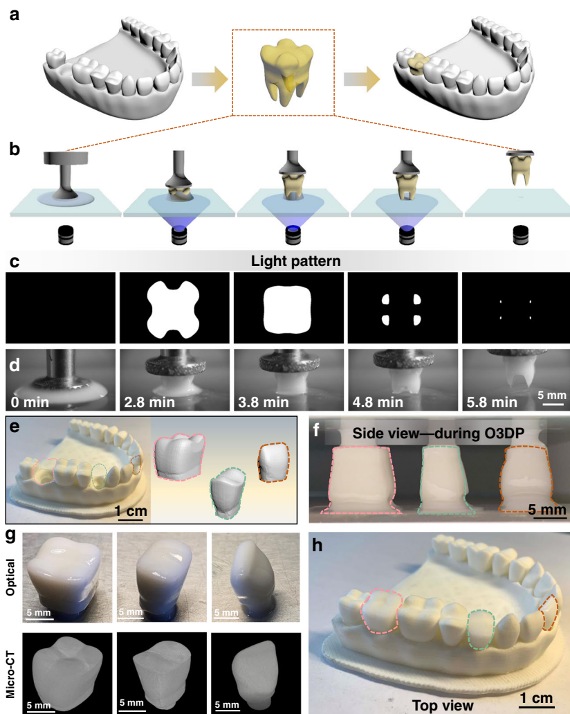
Fig. 4 Fine tooth structure fabricated through the one-droplet 3D printing process. a Scheme of the generation of the tooth model for the one-droplet 3D printing process. b, c Schemes ( b ), UV pattern sequences ( c ) and corresponding optical images ( d ) of the one-droplet 3D printing process, in which a resin droplet is cured into a desired tooth structure. e Scheme of the three selected crown structures and corresponding opposing dentition. Pink, green and orange indicate the crowns of a molar, a canine and an incisor. f Optical image of the one-droplet 3D printing process for printing artificial crown structures. g Optical and micro-CT characterization of the printed crown structures, including the printed molar, canine, and incisor crowns structures. h Fixation of the printed crowns into the model with opposing dentition, with appropriate contact with adjacent teeth and marginal integrity.
