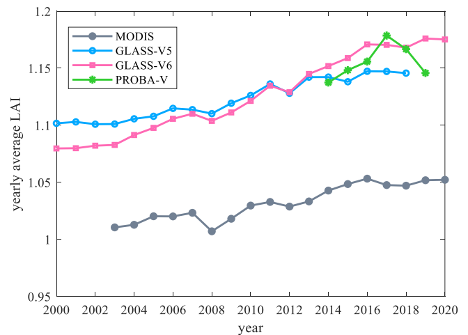
Fig. 14. Variations of the yearly average LAI values from 2000 to 2020 of the MODIS, PROBA-V, GLASS V5, and V6 products for the land surface between 70° N and - 60°S.
