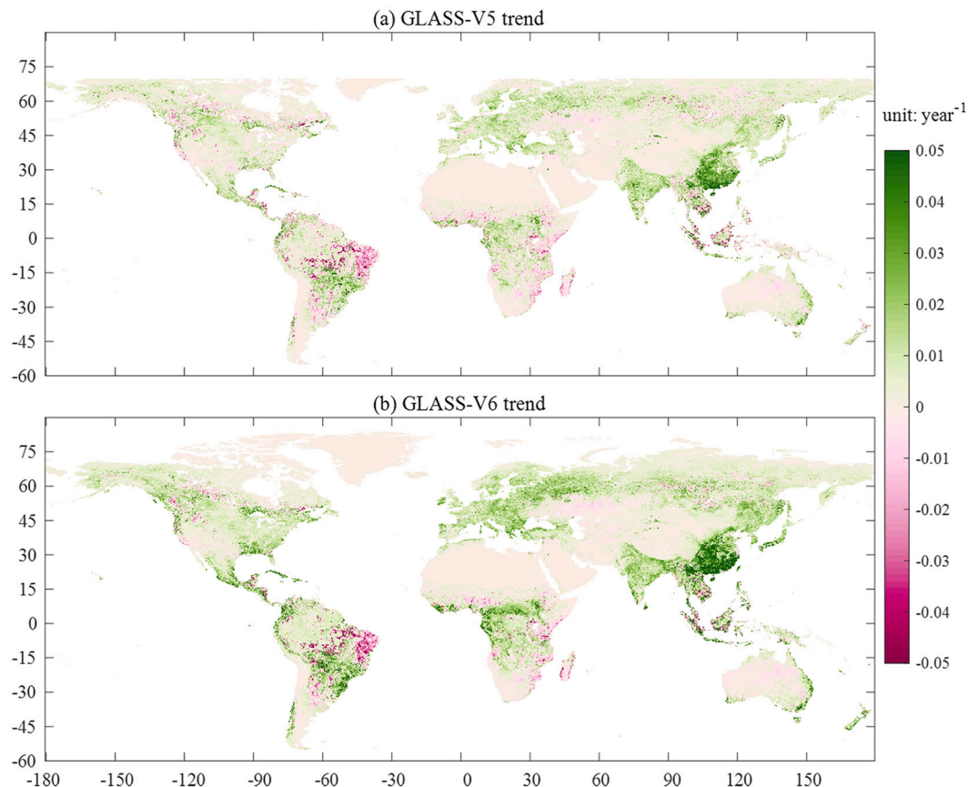
Fig. 13. Slope of the regression line fitting the temporal curve of the annual average LAI (a) GLASS V5 and (b) V6 products from 2000 to 2018; the spatial resolution is 0.05° in geographic latitude/longitude.
