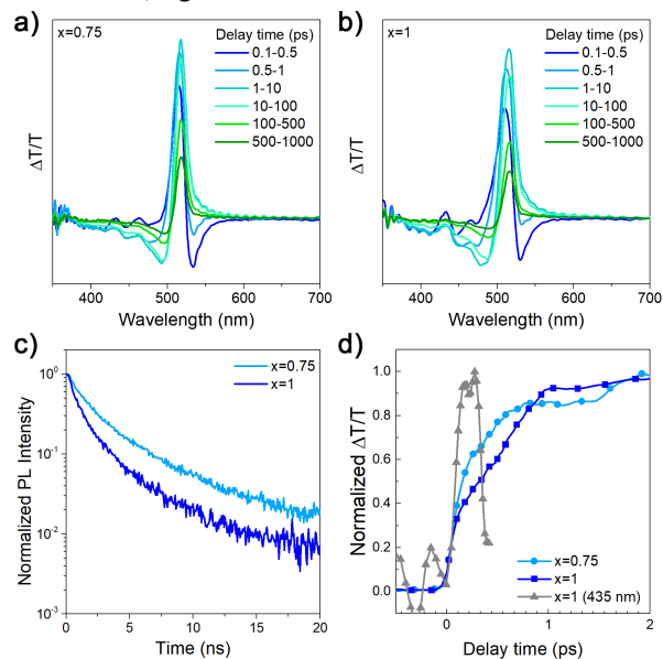
Figure 3. a-b) Transient absorption spectra and c) time resolved PL spectra of (\text{DDA}_x\text{HDA}_{1-x})\text{Cs}_{n-1}\text{Pb}_n\text{Br}_{3n+1} films with x=0.75 and 1 , respectively; d) TA kinetics probed at the peak wavelengths \sim 518 nm and \sim 516 nm for x=0.75 and x=1 respectively. The normalized kinetics of x=1 sample probed at 435 nm ( n=2 ) peak in grey, shows its fast increase within the pulse resolution in comparison to the slower growth of the GSB probed at the quasi-3D peak of x=1 sample in dark blue.
