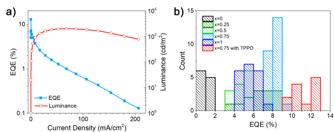
Figure 4. a) Luminance and EQE as a function of current density for (\text{DDA}_{0.75}\text{HDA}_{0.25})\text{Cs}_{n-1}\text{Pb}_n\text{Br}_{3n+1} based LED device with TPPO passivation; b) EQE histograms of (\text{DDA}_x\text{HDA}_{1-x})\text{Cs}_{n-1}\text{Pb}_n\text{Br}_{3n+1} based LED devices with various DDA content x and passivation conditions
