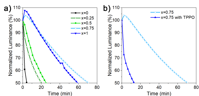
Figure 5. a) Lifetime of (\text{DDA}_x\text{HDA}_{1-x})\text{Cs}_{n-1}\text{Pb}_n\text{Br}_{3n+1} based LED devices with various DDA content x and b) x=0.75 with and without TPPO passivation. The lifetime of all devices were characterized with an initial luminance of 100 \text{cd}/\text{m}^2 .
