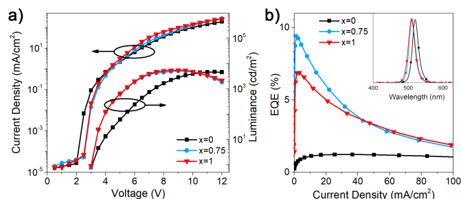
Figure 2. a) J-V-L curves of (\text{DDA}_x\text{HDA}_{1-x})\text{Cs}_{n-1}\text{Pb}_n\text{Br}_{3n+1} based LED devices with x=0, 0.75 , and 1 , respectively. b) EQE versus current density of (\text{DDA}_x\text{HDA}_{1-x})\text{Cs}_{n-1}\text{Pb}_n\text{Br}_{3n+1} based LED devices with x=0, 0.75 , and 1 , respectively. The inset shows the normalized EL spectra of the corresponding devices.
