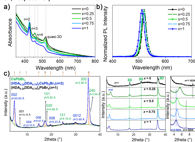
Figure 1. a) Absorption spectra (with indicated peak positions corresponding to different phases), b) normalized PL spectra and c) X-ray diffraction patterns of (DDA x HDA 1- x )Cs n-1 Pb n Br 3 n+1 films with different DDA content x .
