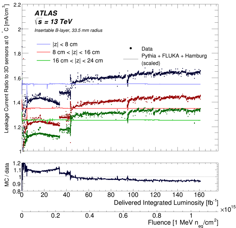
Figure 5. The measured and predicted leakage currents on the Insertable B -layer, both normalized to 0\text{ }^{\circ}\text{C} , divided by the currents in the 3D modules at 24 < |z| < 32\text{ cm} . The other three module groups represent |z| < 8\text{ cm} , 8 < |z| < 16\text{ cm} , and 16 < |z| < 24\text{ cm} . The A and C sides of the detector ( z > 0 and z < 0 ) are consistent with each other and averaged. The dominant time-independent uncertainty of 10% is not included to avoid overlapping bands. The prediction is based on the thermal history of the modules combined with the Hamburg Model for modelling changes in the leakage current and PYTHIA + FLUKA for simulating the overall fluence. For all four predictions, the overall scale normalization is based on a fit to the data across the entire range. Normalization factors are determined per |z| region. The lower panel shows the ratio of the prediction to the data for the innermost module group. Similar MC/data trends are observed for the other three |z| regions. For illustration, the fluence is shown as a lower horizontal axis using the nominal luminosity-to-fluence from simulation at |z| = 0 .
