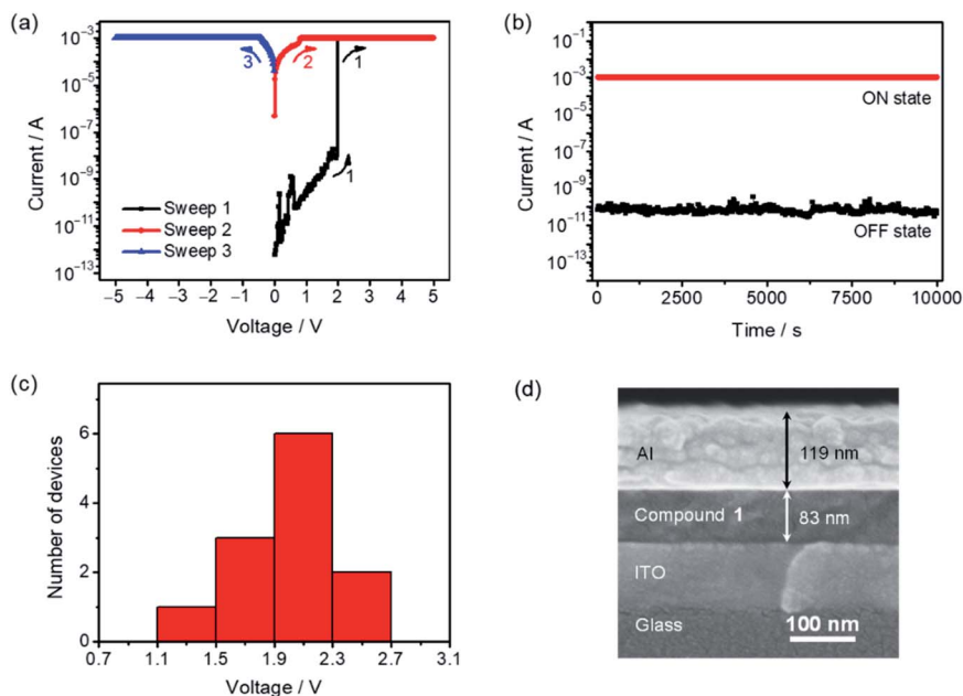
Fig. 7 (a) I-V characteristics, (b) retention time in “OFF” and “ON” states under a constant bias of 1 V, (c) distribution of the switching threshold voltage (12 devices) and (d) SEM image of the cross-section of the memory device fabricated with 1 .
