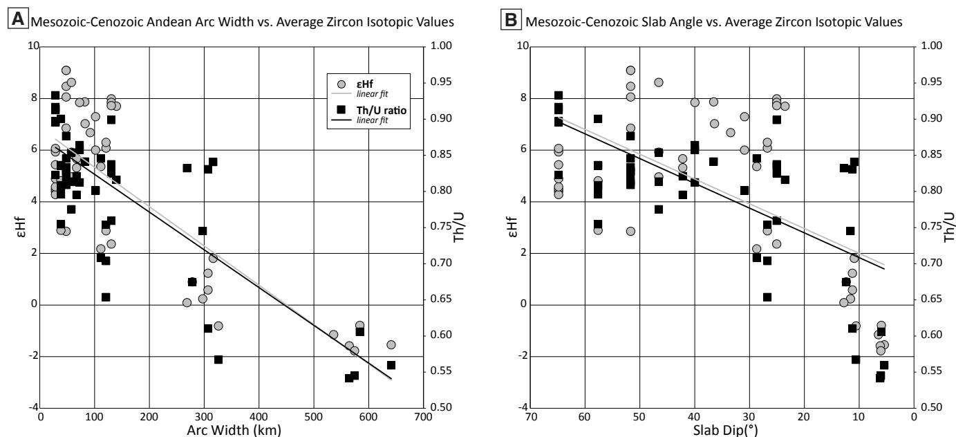
Figure 11. Comparisons of Mesozoic–Cenozoic Andean arc width, subduction angle, and zircon composition along Argentina and Chile (28.5°S to 33°S). (A) Andean arc width relative to zircon \epsilon_{\text{Hf}} and Th/U values (Table S5 [see text footnote 1]). (B) Subduction angle relative to zircon \epsilon_{\text{Hf}} and Th/U values (Table S5 [see text footnote 1]).
