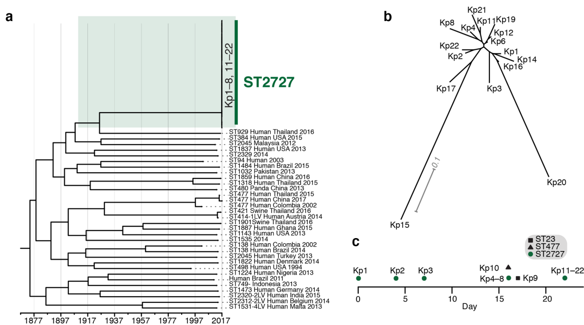
Fig. 1. Genomic epidemiology and timeline of K. quasipneumoniae subsp. similibremoniae . (a) Evolutionary relationships and timescale of evolution of 54 K. quasipneumoniae subsp. similibremoniae (KpIIB) strains. (b) Phylogenetic tree of the ST2727 isolates collected in the NICU during February and March 2017. The phylogenetic tree was built using the BioNJ algorithm on SplitsTree. Scale bar represents nucleotide substitutions per site. (c) Timeline of sample collection in the NICU, where calendar dates have been replaced by a timeline where the first sample was collected on day 0.
