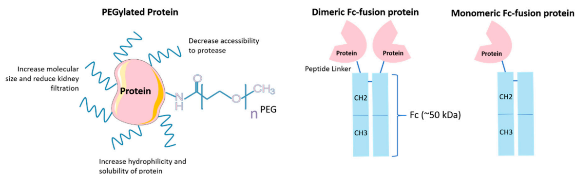
Figure 4. Structure of PEGylated protein and Fc-fusion protein. PEGylation is a chemical process involving the attachment of polyethylene glycol (PEG) chains to a molecule of interest through covalent binding or non-covalent complexation; Fc-fusion proteins are composed of the Fc domain of IgG genetically linked to a peptide or protein of interest. The first-generation Fc-fusion proteins are dimeric wherein an effector molecule is fused with each arm of the Fc fragment. The second-generation Fc-fusion proteins are monomeric wherein a single effector molecule is conjugated to one arm of the Fc fragment.
