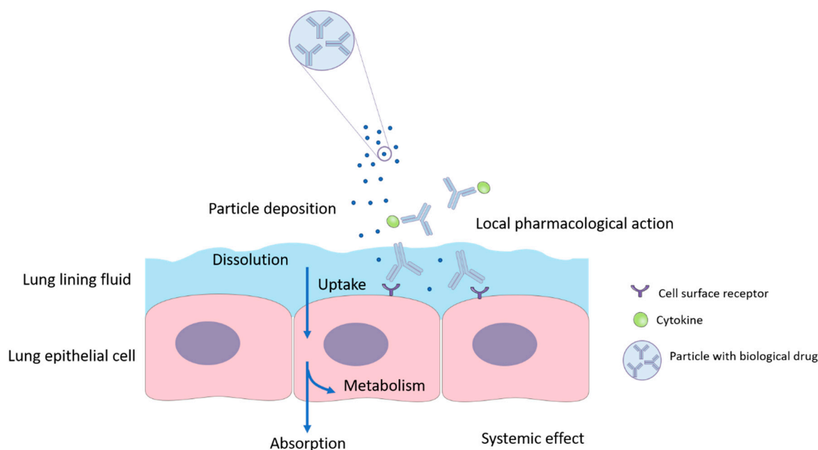
Figure 1. The fate of inhaled biological drugs in the airways upon lung deposition. Following dissolution in the lining fluid, the biological drugs either act on the surface of the epithelial cells, or being taken up by the cells where they are metabolised or absorbed into the systemic circulation.
