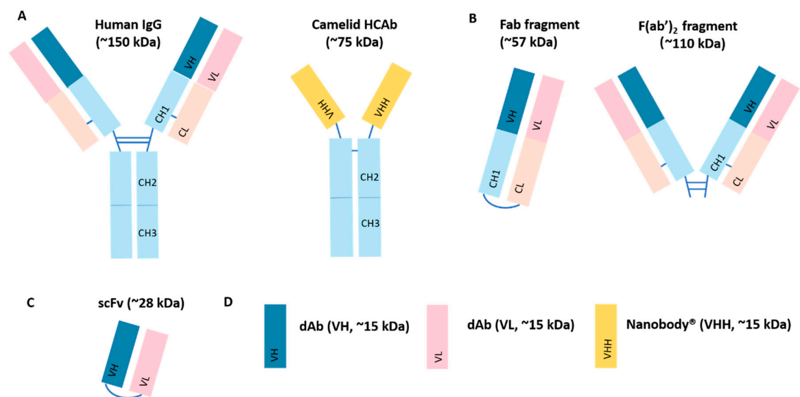
Figure 3. Schematic representation of different antibody fragments investigated for pulmonary delivery. (A) Conventional antibodies from mammals have Y-shape structure composed of two identical heavy and light chains. Each chain contains constant regions (CH1, CH2, CH3 and CL) and variable regions (VH and VL) that are held together by disulfide bonds. Members of the Camelidae family naturally produce a unique type of immunoglobulin that is devoid of light chains. These heavy chain-only antibodies (HCAbs) are formed by a single variable domain (VHH) and two constant domains; (B) Fab is an antibody fragment that can bind to antigens without Fc region; F(ab') 2 contains two Fab fragments linked together by disulfide bonds; (C) Single-chain fragment variable (scFv) is composed of variable domains of the heavy (VH) and light chains (VL) of human IgG, connected by a peptide linker; (D) Domain antibodies (dAbs) are antibody fragments derived from the variable domains of either the heavy or light chain of human IgG. Nanobody ® is the recombinant single-domain antibody derived from the HCAbs of Camelidae.
