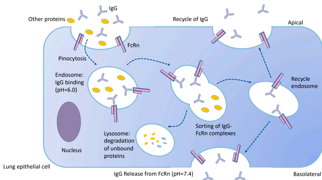
Figure 2. Transport and recycle of IgG in the lung epithelium by the FcRn-mediated pathway. IgG is taken up into FcRn-expressing epithelial cells via non-specific fluid-phase pinocytosis. IgG then binds to the transport receptor, FcRn, which is mainly distributed within the acidic endosomal vesicles in the cell. The Fc receptor binds to IgG with high affinity at low pH but shows no affinity at physiologic pH. FcRn with bound IgG is sorted into the sorting endosome, which either recycle or transcytose to the plasma membrane. Nonprotected IgG and proteins proceed to lysosomal proteolytic degradation. The near-neutral pH results in dissociation and release of IgG from FcRn into the extracellular fluid.
