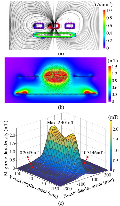
Fig. 13. Magnetic field distributions. (a) Flux lines and current densities. (b) Flux densities along the vertical plane. (c) 3-D flux densities along the parallel plane.
