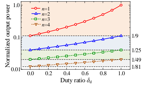
Fig. 9. Normalized output power versus duty ratio with different n under the PFM.
