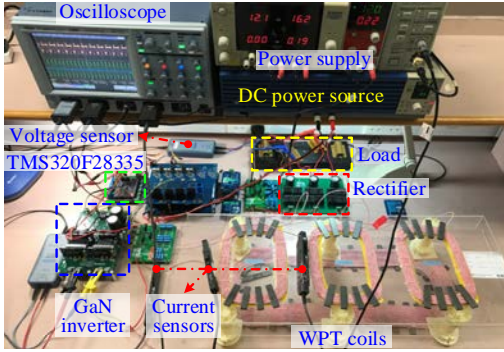
Fig. 15. Experimental setup.
