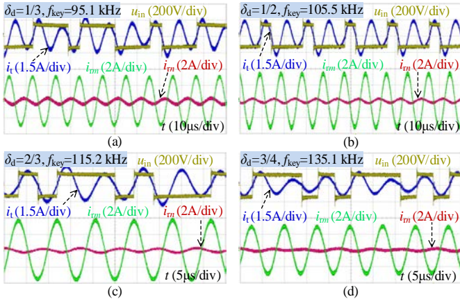
Fig. 16. Measured waveforms of the multi-objective WPT system using proposed soft-switching PFM. (a) \delta_d=1/3, f_{key}=95.1 kHz. (b) \delta_d=1/2, f_{key}=105.5 kHz. (c) \delta_d=2/3, f_{key}=115.2 kHz. (d) \delta_d=3/4, f_{key}=135.1 kHz.
