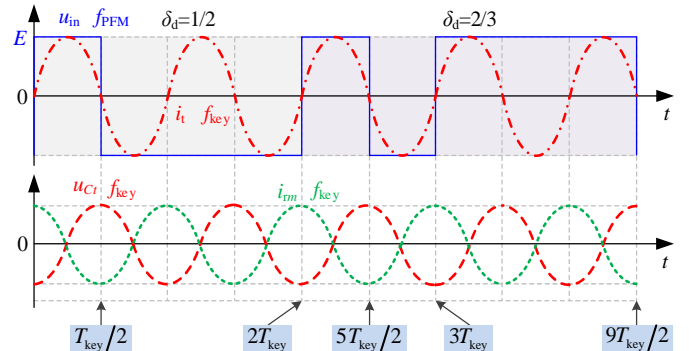
Fig. 3. Theoretical waveforms of proposed soft-switching PFM-WPT.
