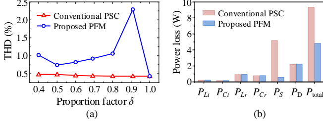
Fig. 14. Characteristic comparisons of the proposed PFM and the PSC. (a) THDs of authorized receiver current. (b) Power losses.
