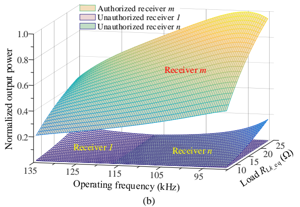
Fig. 10. Wireless power characteristics of proposed PFM-WPT system. (a) Selectivity. (b) Security.
