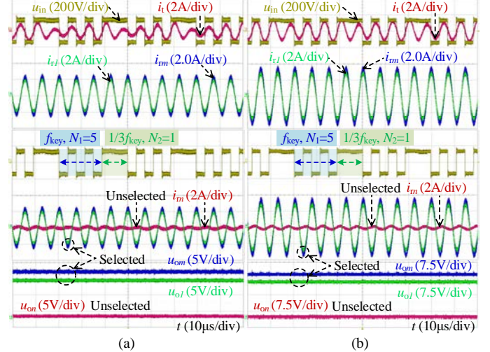
Fig. 18. Measured waveforms of proposed simultaneously multi-objective PFM-WPT. (a) No misalignment. (b) 50% misalignment.
