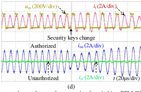
Fig. 17. Measured waveforms of proposed soft-switching PFM-WPT system. (a) Wireless energy selectivity when left lateral receiver selected. (b) Wireless energy selectivity when middle receiver selected. (c) Wireless energy security. (d) Transient energy transfer process when the security keys change.
