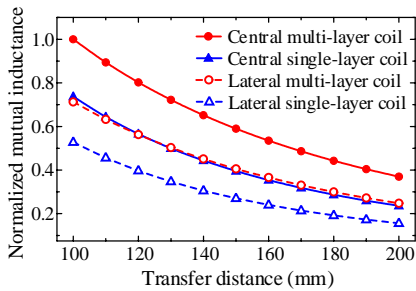
Fig. 12. Normalized mutual inductances versus transfer distance.
