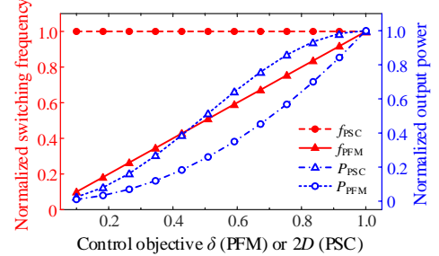
Fig. 8. Normalized average switching frequency and wireless power controllability under proposed soft-switching PFM and conventional PSC.
