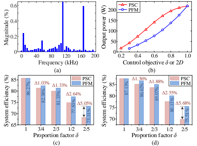
Fig. 19. Measured characteristics of proposed full-range soft-switching PFM-WPT system. (a) FFT result of receiver current. (b) Wireless energy controllability. (c) Overall system efficiencies when middle receiver selected. (d) Overall system efficiencies when lateral receiver selected.
