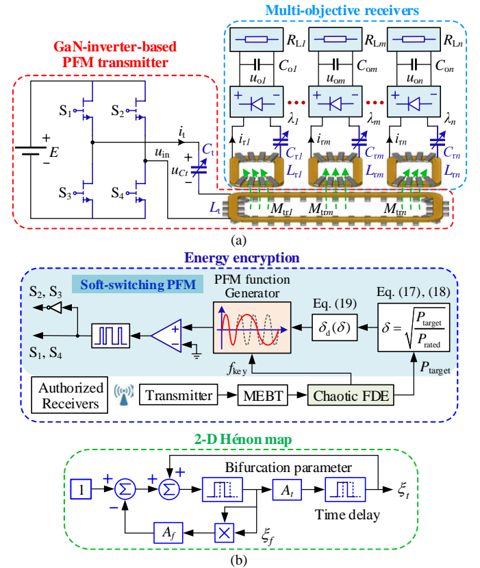
Fig. 1. Multi-objective GaN-inverter-based WPT system using proposed soft-switching PFM with controllability, selectivity and security. (a) Topology. (b) Soft-switching PFM and 2-D chaotic energy encryption.
