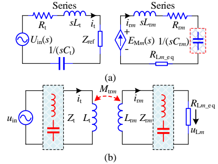
Fig. 4. Equivalent circuits. (a) Exemplified SS topology in the complex frequency domain. (b) Multi-topological compensation networks.
