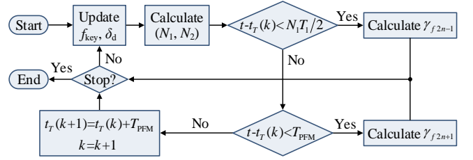
Fig. 20. Algorithm of proposed PFM function generator.
