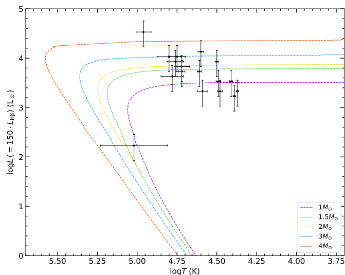
Figure 1. A Hertzsprung-Russell diagram for Galactic Bulge CSPNe from this work. Evolutionary tracks by Miller Bertolami [2] are also shown for reference. The error bars for each luminosity correspond to the range of values for the adopted distance of 8.5 \pm 2.5 kpc for the Galactic Bulge. Rough estimates to the upper and lower limits for the Zanstra temperature are provided. The wide range of temperature for H 2–15 (CSPN on the white dwarf cooling track) reflects the large uncertainties in the HST photometry for this CSPN.
