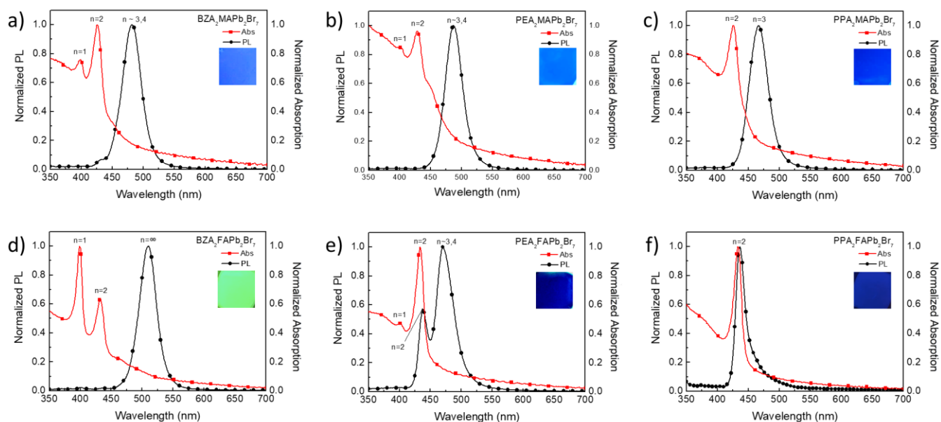
Fig. 1 Absorption and PL spectra of a) \text{BZA}_2\text{MAPb}_2\text{Br}_7 , b) \text{PEA}_2\text{MAPb}_2\text{Br}_7 , c) \text{PPA}_2\text{MAPb}_2\text{Br}_7 , d) \text{BZA}_2\text{FAPb}_2\text{Br}_7 , e) \text{PEA}_2\text{FAPb}_2\text{Br}_7 and f) \text{PPA}_2\text{FAPb}_2\text{Br}_7 . The insets show corresponding photos of the films under UV illumination.
