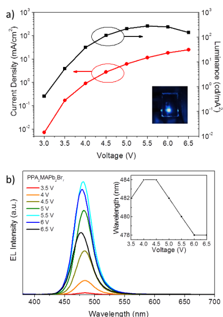
Figure 3 a) L-I-V plots (device photo is shown in the inset) and b) EL spectra vs. bias voltage for \text{PPA}_2\text{MAPb}_2\text{Br}_7 devices. The center wavelength position as a function of bias voltage is shown in the inset.
