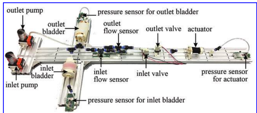
FIG. 6. CSB testing platform setup. Color images are available online.
