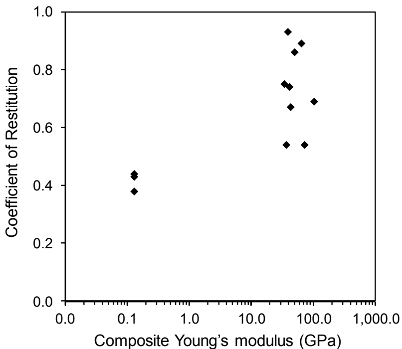
72 Figure 13. Variation of the average values of coefficient of restitution with composite 73 Young's modulus of the grain and base block combinations whole set of data)
