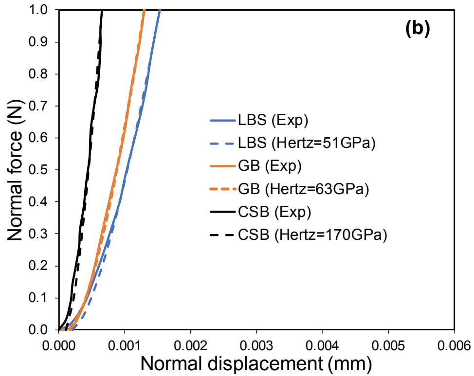
Figure 2. a) Photograph of chrome steel balls during application of normal force using inter-particle loading apparatus b) The typical normal force against displacement behaviour along with Hertzian fitting for the spheres tested in this programme
