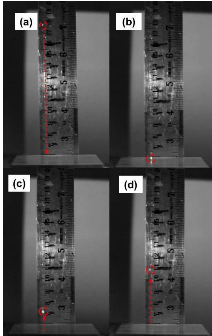
Figure 5. Various stages of chrome steel ball impacting on stainless steel surface a) Initial path of drop b) Impacting the surface of stainless steel c&d) Rebound path
