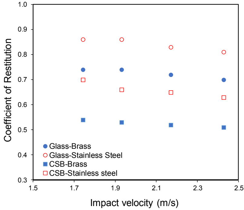
44 Figure 7: The coefficient of restitution against impact velocity for GB and CSB on brass and 45 stainless steel blocks
