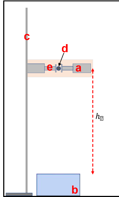
Figure 4. Schematic side view of the drop test apparatus a) Solenoids holding the particle b)
