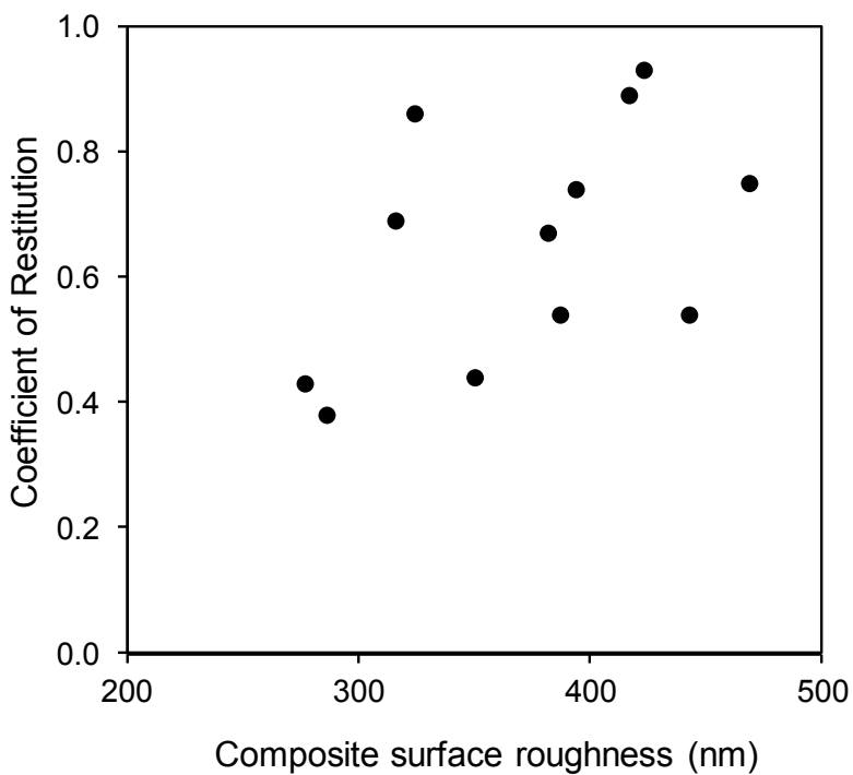
76 Figure 14. Variation of the average values of coefficient of restitution with composite 77 surface roughness of the grain and base block combinations data excluding rubber block)
