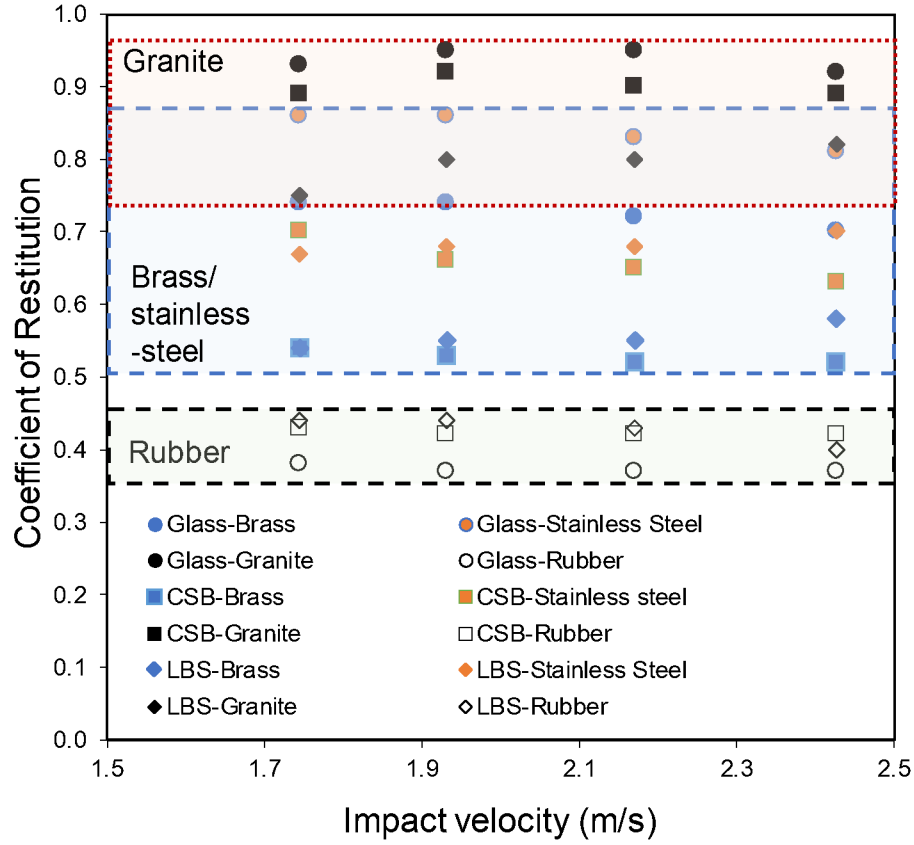
Figure 12. The average values of coefficient of restitution for all the grain and base block combinations
