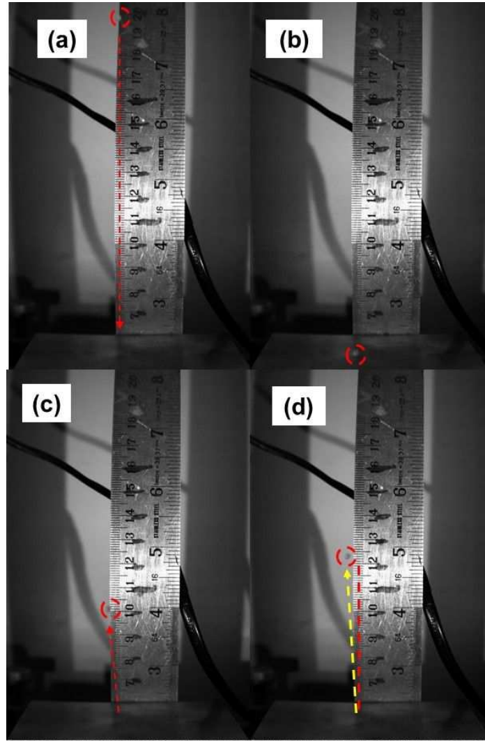
Figure 9. Various stages of LBS impacting on surface of brass block surface a) Initial path of drop b) Impacting the surface of brass block c&d) Rebound path
