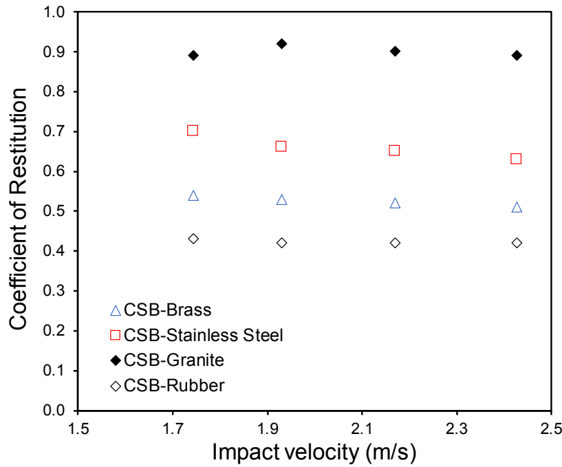
47 Figure 8: The coefficient of restitution against impact velocity for CSB on different base 48 blocks
