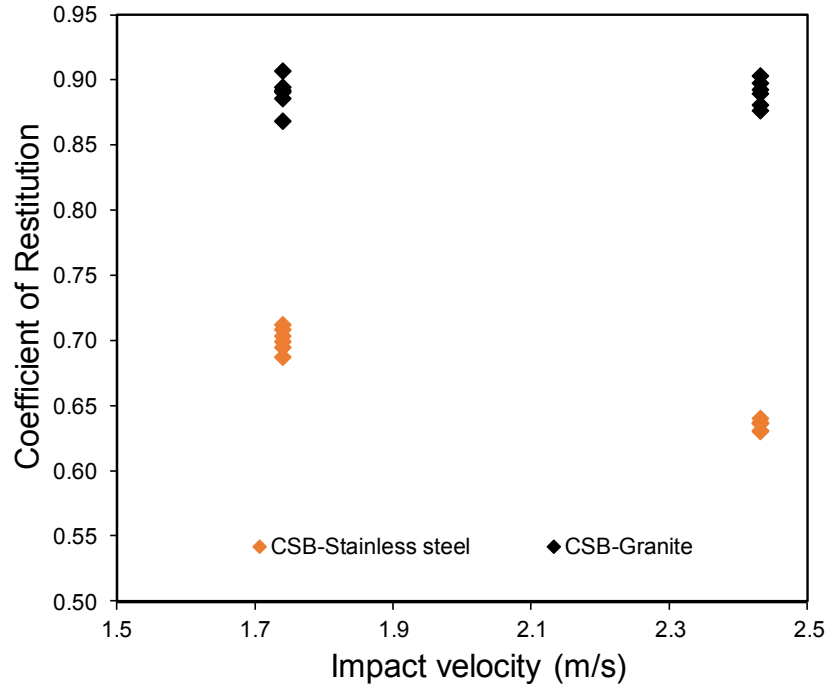
Figure 6: The repeatability of the coefficient of restitution values for CSB impacting on stainless steel and granite blocks
