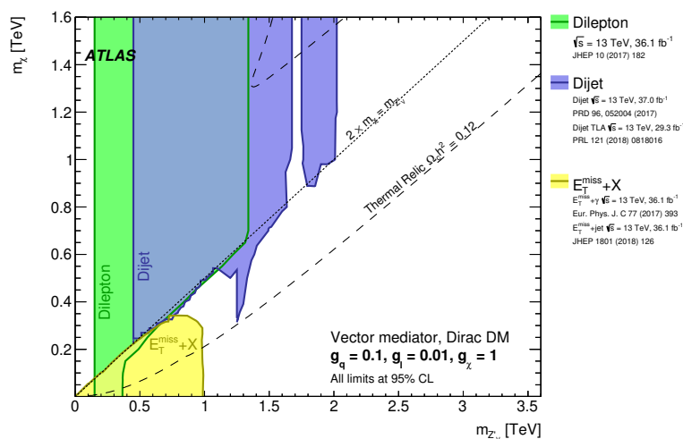
Figure 11. Regions in a (mediator-mass, DM-mass) plane excluded at 95% CL by dijet, dilepton and E_T^{\text{miss}} + X searches, for leptophobic (a) or leptophilic (b) vector mediator simplified models described in section 2.1.1. The exclusions are computed for a DM coupling g_\chi , quark coupling g_q , universal to all flavours, and lepton coupling g_\ell as indicated in each case. Dashed curves labelled “thermal relic” correspond to combinations of DM and mediator mass values that are consistent with a DM density of \Omega h^2 = 0.12 and a standard thermal history as computed in MadDM [77, 204]. Above the curve in (a) annihilation processes described by the simplified model deplete \Omega h^2 to below 0.12. In (b), this occurs between the two dashed curves. The dotted line indicates the kinematic threshold where the mediator can decay on-shell into DM.
