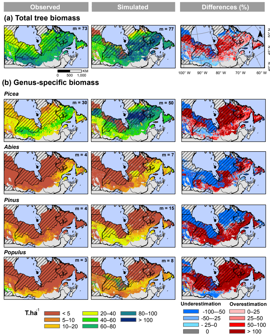
Figure 4. (a) Observed, LPJ-LMfire simulated, and differences (%) in mean total aboveground biomass ( \text{T ha}^{-1} ) between 2000 and 2006 across eastern boreal Canada. (b) Genus-specific aboveground biomass. The observed aboveground biomass maps across Canada were predicted and validated with photo-plot information in the southern areas (non-hatched areas) and data published by Beaudoin et al. (2014). Median ( m ) tree aboveground biomass values are also indicated for each map; these were calculated for the non-hatched areas at a 10 km resolution.
