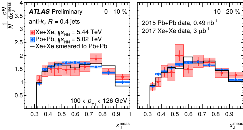
Fig. 2. The 1/N dN/dx_J^{\text{meas}} distributions for jet pairs with 100 < p_{T,1} < 126 GeV in 0–10% and 10–20% centrality intervals. The Xe+Xe data are shown in circles, while the Pb+Pb distribution is shown for comparison in diamonds. Statistical uncertainties are indicated by the error bars while systematic uncertainties are shown with shaded boxes. The Xe+Xe systematic uncertainties include all of the JES and JER uncertainties on Xe+Xe data. The Pb+Pb systematic uncertainties include only the uncertainties that are uncorrelated between Xe+Xe and Pb+Pb collisions. The black line represents the inclusion of additional underlying event fluctuations based on the results of the fluctuations analysis. Figure taken from [4].
