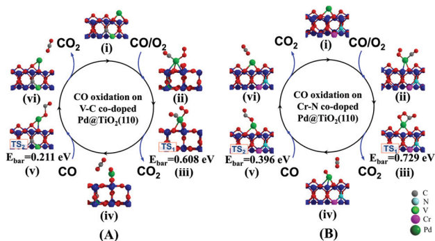
Fig. 6 Minimum energy paths for CO oxidation on \text{Pd}@\text{TiO}_2(110) co-doped with prototypical metal–nonmetal pairs. (A) p-Type V–C and (B) n-type Cr–N co-dopants.
