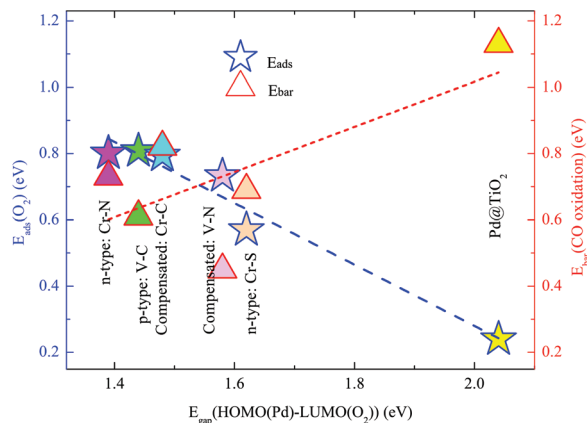
Fig. 5 Adsorption energy of the O_2 molecule, E_{\text{ads}}(O_2) (activation barrier for CO oxidation, E_{\text{bar}}(\text{CO oxidation}) ) on \text{Pd}@\text{TiO}_2(110) and co-doped counterparts with V–C, V–N, Cr–C, Cr–N, and Cr–S co-dopant pairs.
