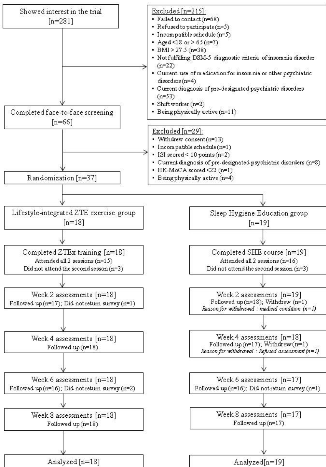
Figure 1. Trial flowchart
