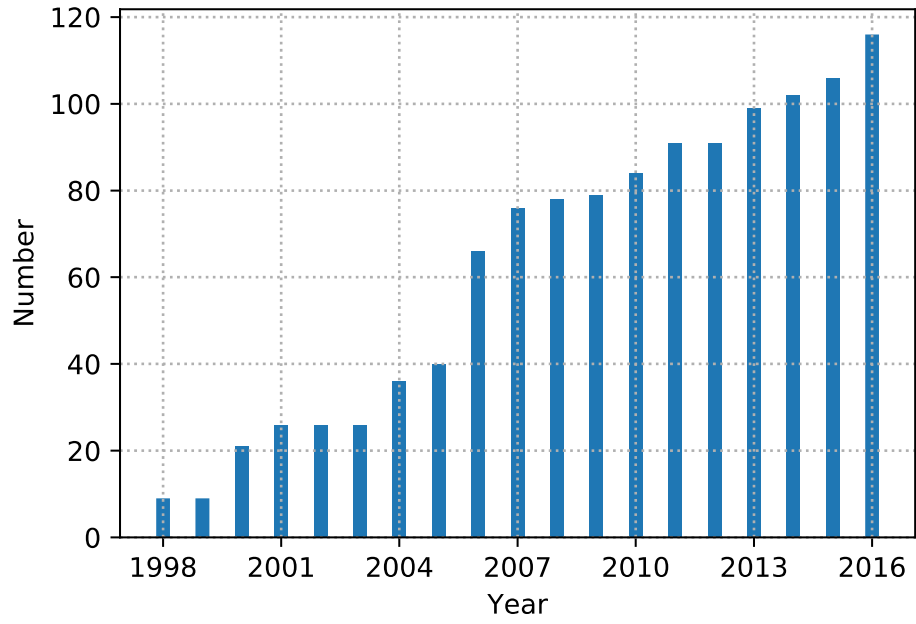
Figure A.1: The number of industry ETFs in our sample over time
