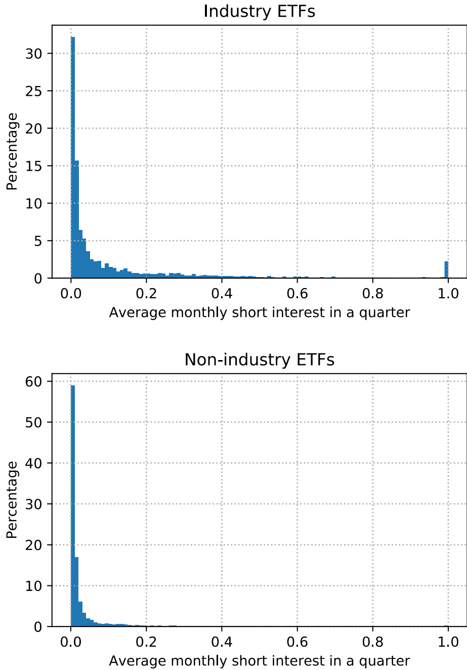
Figure 2: The histogram of the short interest ratio
