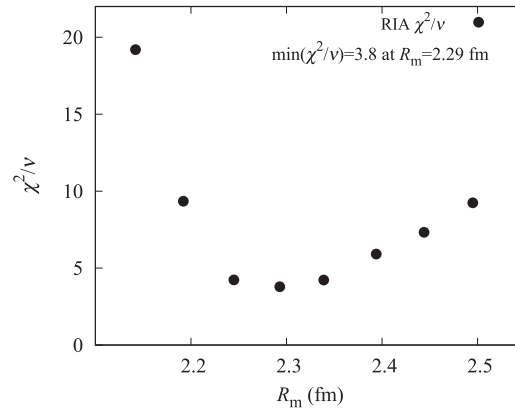
Fig. 9. The distribution of the reduced \chi^2 value ( \chi^2/\nu , vertical axis) as a function of the matter radius (horizontal axis) of the RIA results of p - {}^6\text{Li} elastic scattering. The best-fit value of R_m = 2.29^{+0.07}_{-0.06} fm.
