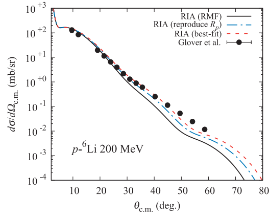
Fig. 8. Results of RIA calculations [18], using initial RMF (solid line), reproducing R_p (dash-dotted line) and best-fit (dashed line) densities of {}^6\text{Li} . The experimental data are from Glover et al. [32] (solid circles). The error bars are comparable with the symbol size.
