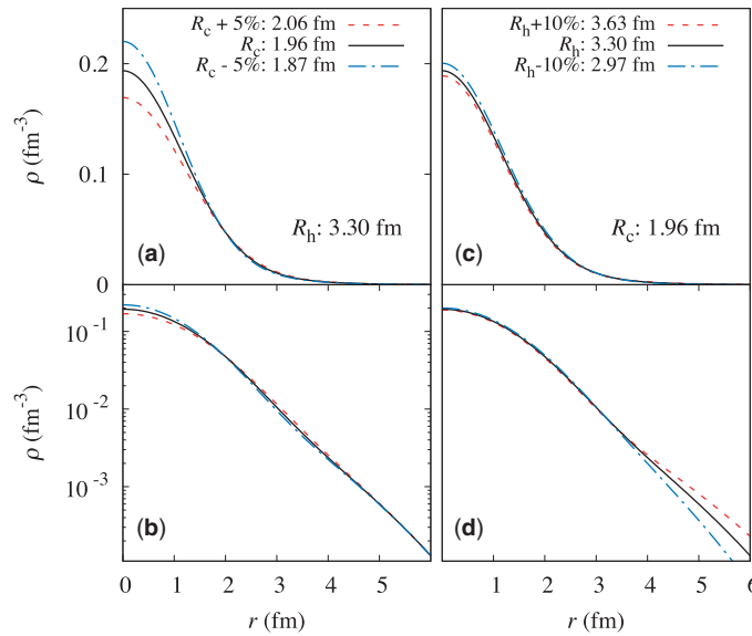
Fig. 10. Total matter density distributions using the GG density model, where RMS radii of core (panels (a) and (b)) and halo (panels (c) and (d)) nucleons were changed by \pm 5\% and \pm 10\% from the initial density deduced in Ref. [17].
