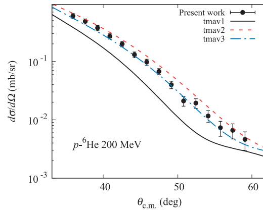
Fig. 14. Results of RIA calculations [18], assuming three RMF-based density distributions of {}^6\text{He} (displayed in Fig. 13) along with the present experimental result of the differential cross sections.
