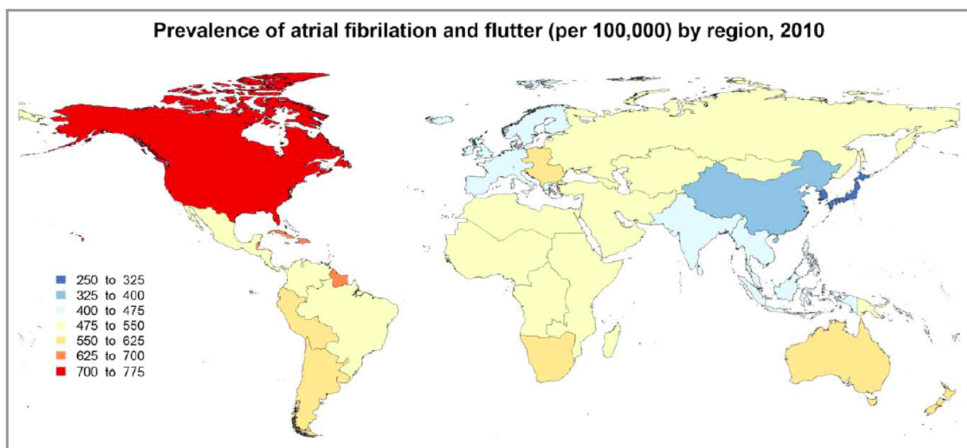
Figure 1. International age-adjusted AF prevalence rates (per 100 000 population) in the 21 Global Burden of Disease regions, 2010. Figure reproduced from Chugh et al 7 with permission from Wolters Kluwer Health, Inc. AF indicates atrial fibrillation.
