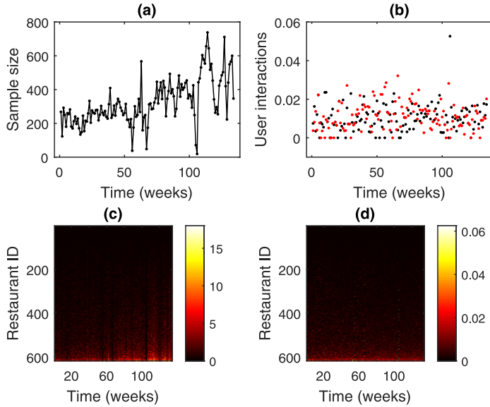
FIG. 4. Description of the raw data over time. (a) Sample size over time; (b) Scatter plot of the proportions of two randomly chosen restaurants over 134 weeks; (c) Heatmap of user interactions of 617 restaurants with brightness representing the frequency of users' final choices; (d) Heatmap of the proportions allotted in all the restaurants with time.
