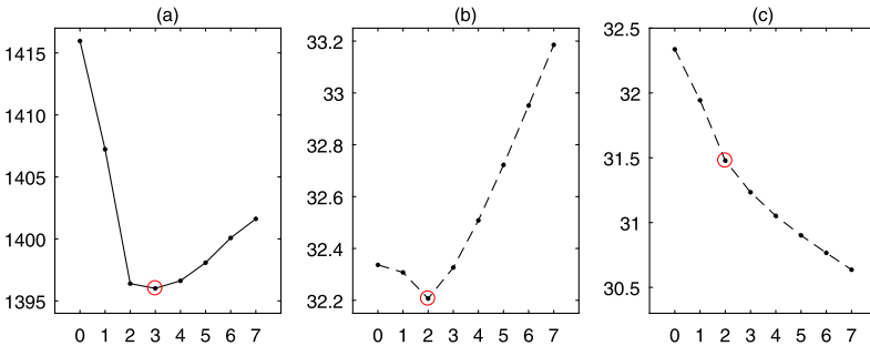
FIG. 6. (a)–(b) Plots of the penalized objective function based on segmentation, corresponding to equations (8)–(9), versus the number of change-points L , respectively. (c) Plot of S_{\hat{\mathcal{B}}}(\hat{\tau}_{L,1}^{(2)}, \dots, \hat{\tau}_{L,L}^{(2)}) + L\hat{Q}_{\hat{\mathcal{B}}}(55, 90) versus the number of change-points L .
