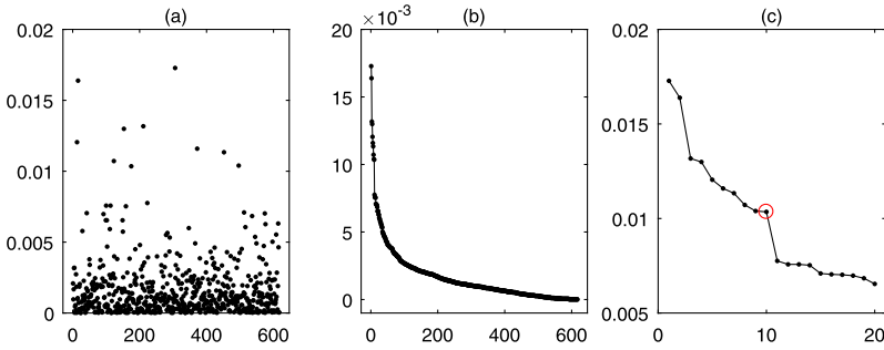
FIG. 5. Estimation of the sparsity pattern. (a) Scatter plot of the estimated proportions \hat{q}_j 's for j = 1, \dots, p ; (b)–(c) Plots of the estimated proportions in a decreasing order, i.e., \hat{q}_{(j)} 's, for j = 1, \dots, p and j = 1, \dots, 20 , respectively.
