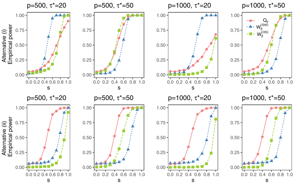
FIG. 2. Comparison of empirical power for the proposed Q_{p, \hat{\mathcal{A}}} test, W_{\hat{p}}^{(SW)} by Srivastava and Worsley (1986) and W_{\hat{p}}^{(HS)} by Horváth and Serbinowska (1995) under the alternative hypothesis (i) with \omega = 0.3 , and the alternative hypothesis (ii) with \omega = 0.7 , where d = 6 .
