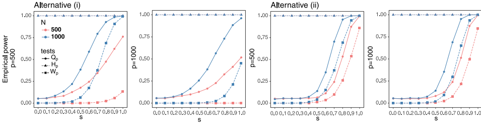
FIG. 1. Comparison of empirical power at a 5% significance level for the two-sample homogeneity test under different (p, N) -settings and the alternative hypothesis (i) with \omega = 0.3 and the alternative hypothesis (ii) with \omega = 0.7 , where d = 6 . Here, Q_p is short for Q_{p, \hat{\mathcal{A}}} .
