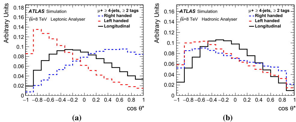
Fig. 3 Templates of the \cos \theta^* distributions for the individual helicity fractions in the \mu + \text{jets} channel with \geq 2 b -tags for the a leptonic and b hadronic analyser
