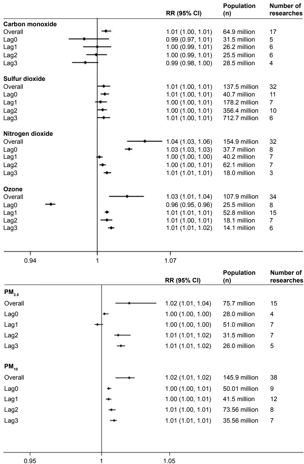
Figure 2 Associations between gaseous and particulate air pollution and COPD risk stratified by time lag (days). Abbreviations: CI, confidence interval; COPD, chronic obstructive pulmonary disease; RR, relative risk.
