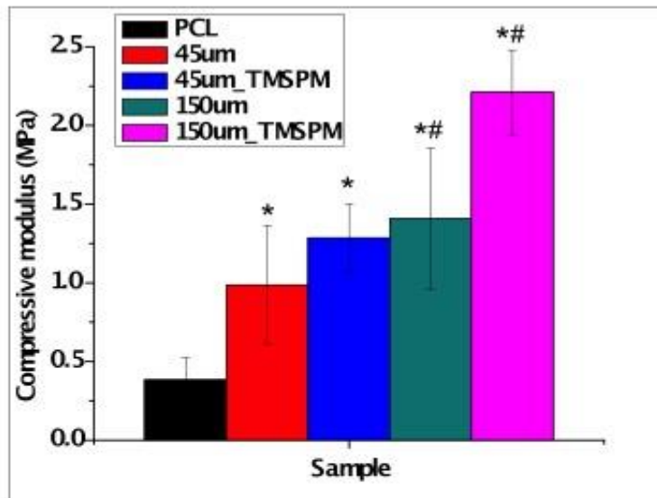
Figure 1 Compressive moduli of the pure PCL porous scaffold, Mg/PCL and silane-coupled Mg/PCL porous scaffolds. The compressive moduli of both the Mg/PCL and silane-coupled Mg/PCL scaffolds were found to be significantly higher ( *p<0.05 ) than the pure PCL scaffold. In addition, the compressive moduli of the silane-coupled 150 \mu\text{m} Mg/PCL porous scaffolds was significantly higher ( ^{\#}p<0.05 ) than the 150 \mu\text{m} Mg/PCL scaffold.
