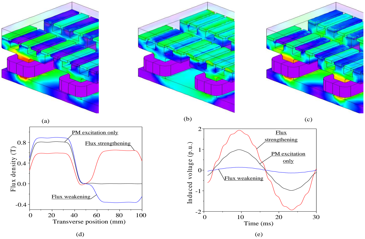
Fig. 2. Analysis results. (a) Field distribution under PM excitation. (b) Field distribution under flux strengthening. (c) Field distribution under flux weakening. (d) Air-gap flux density. (e) No-load induced voltage waveforms.
